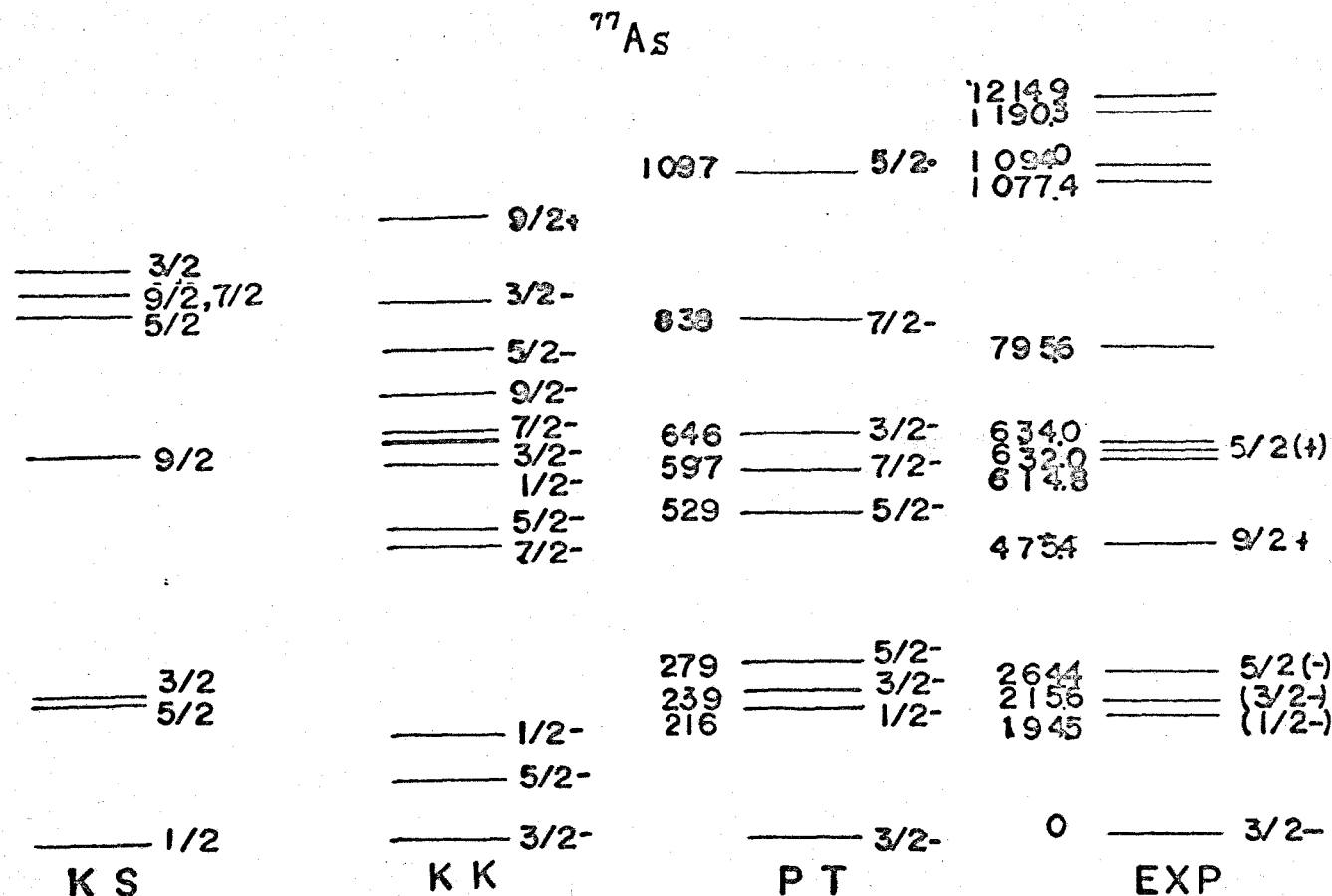
Fig. 5-12. Comparison of the theoretical level energies in ^{77}\text{As} with those obtained by experiment (marked EXP). Present theoretical level energies (marked PT) are obtained for \eta = 6 and \frac{\hbar^2}{2\theta} = 60 keV. Previous theoretical works done by Kisslinger and Sorensen and by Kisslinger and Kumar are marked KS and KK, respectively.
