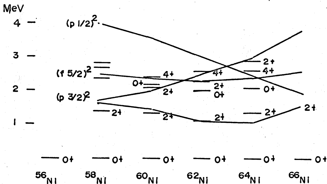
Fig. 4-3. Energy levels of doubly-even-mass Ni isotopes. Horizontal lines are the experimental levels and solid lines join the theoretical ones calculated for G = 19/A MeV.
