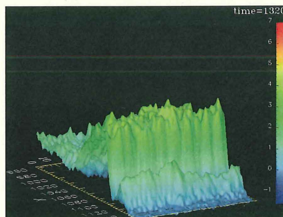
Fig.1: 3D Plot of magnetic field issued from full Particle numerical Simulation which help to reproduce artificially and to analyze the natural Terrestrial bow shock (large jump on the figure) in space plasmas. Such simulations require very large scale supercomputers.
