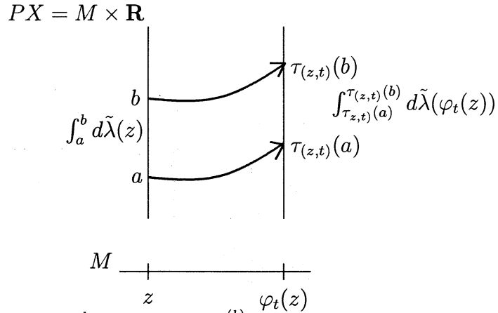
Figure 5: \int_a^b d\tilde{\lambda}(z) = \int_{\tau_{(z,t)}(a)}^{\tau_{(z,t)}(b)} d\tilde{\lambda}(\varphi_t(z))
