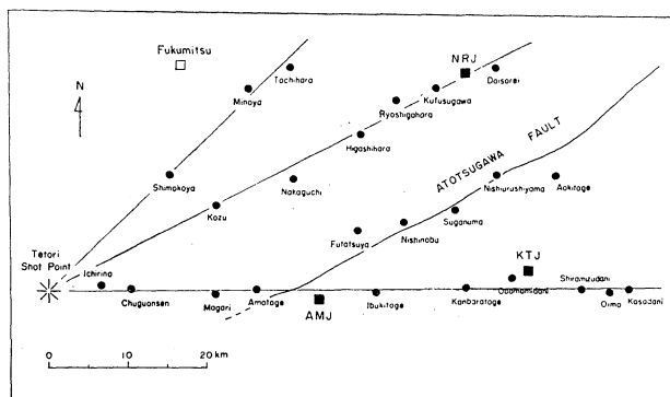
Fig. 1. Location of temporary observation sites for the Totori quarry blasts (solid circles) and routine seismograph stations (solid squares), KTJ; Kamitakara, AMJ; Amo and NRJ; Nirehara.
