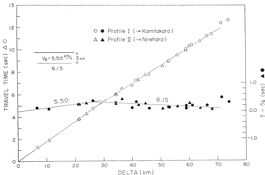
Fig. 2. Observed travel times (open symbols) and the corresponding reduced times T-\Delta/v (solid symbols) from the Totori quarry blasts. Apparent velocities and the upper crustal structures are also indicated.
