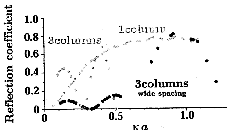
Fig. 4 Reflection coefficient.
