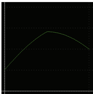
Figure 3: B_1 = \{\|k\| = 1\} , A = \text{co}\{(3, 1), (2, 2)\}
