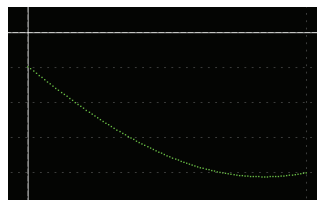
Figure 4: A = \{(-4, -1)\}
