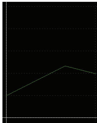
Figure 2: A = \{\text{co}\{(3, 1), (2, 3)\}\}
