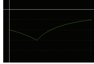
Figure 6: Nonlinear, A = \{(-1, -2)\}
