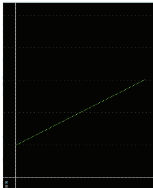
Figure 1: A = \{(3, 1)\}
