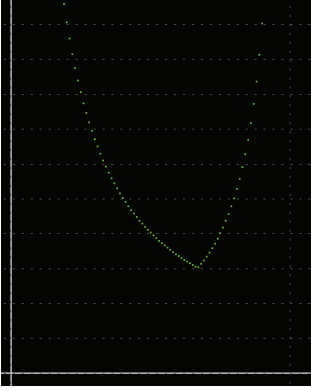
Figure 5: Nonlinear, A = \{(2, 1)\}
