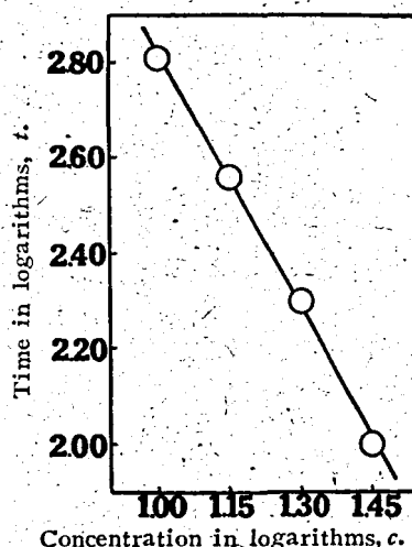
Fig. 2. The relation between log time and log concentration at the 50 per cent knock down, the equation of the straight line in original units is C^{1.791} t = 40821 .
