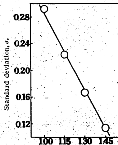
Fig. 3. Relation of the standard deviation \sigma , or 1/\text{slope} to the log-concentration c of \alpha -dl-trans-allethrin from Table 4, the equation of the straight line in corrected value is \sigma_a = 0.63527 - 0.35761c
