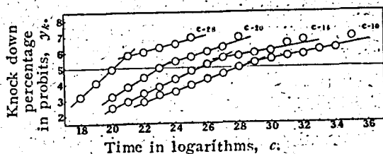
Fig. 1. Time-knock down regression isodose in the range of concentration of \alpha -dl-trans-allethrin C from 10 to 28 (10mg./10g.).
