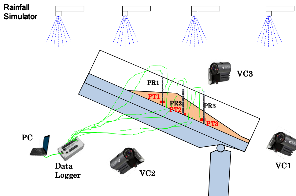
Fig. 2 Experimental setup
