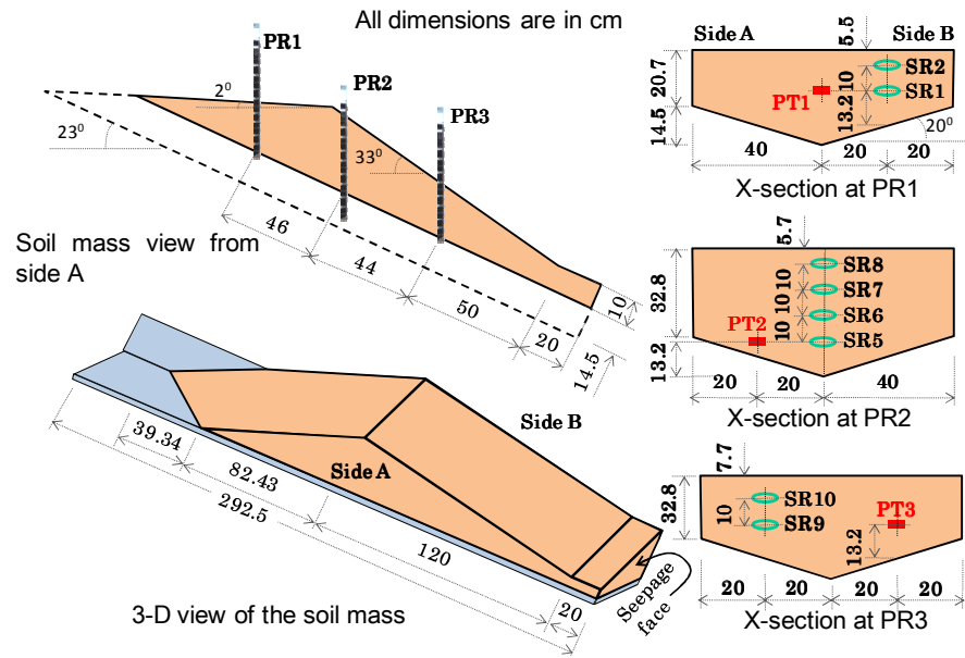
Fig. 3 Shape and size of the model slope with the arrangement of SRs and PTs
