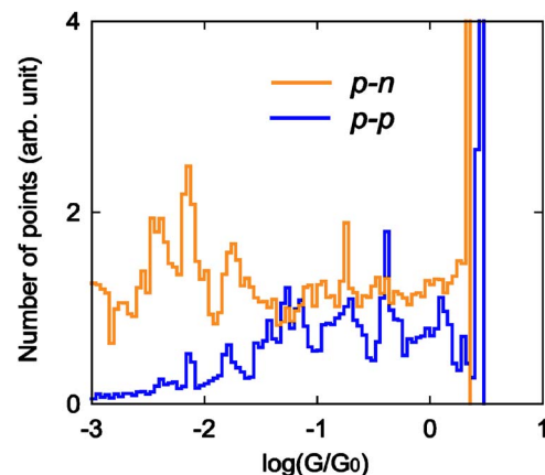
FIG. 3. (Color online) The p-n and the p-p conductance histograms at +2 V in the high-conductance region G > 10^{-3}G_0 . The histograms are plotted against \log(G/G_0) to cover the wide distribution of the junction conductance. A few peaklike features are commonly observed in two histograms.
