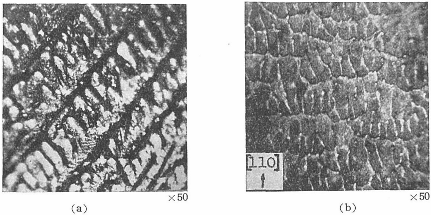
Fig. 9. Microstructures of the sectional surfaces of the specimen shown in Fig. 4. (a) (001) plane etched electrolytically. (b) ( \bar{1}\bar{1}0 ) plane etched electrolytically.
