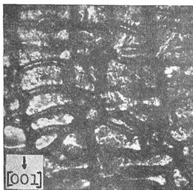
Fig. 2. Microstructure of top free surface of the specimen shown in Fig. 1, (100). Lowering speed, 1 mm/min.
