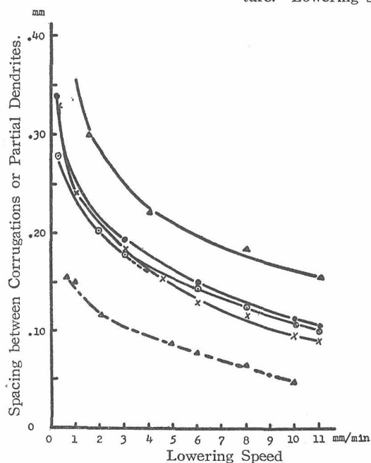
Fig. 6. Spacing between corrugations or partial dendrites vs. lowering speed. \blacktriangle , Direction of growth is parallel to [100] ; \bullet , inclines at 30^\circ from [110] to [100] ; \odot , inclines at 20^\circ from [110] to [100] ; \times , inclines at 10^\circ from [110] to [100] . Chain line corresponds to side arms.
