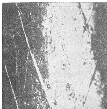
Fig. 12. Microstructure of side surface of the specimen, (001), which was grown in the direction inclined at 20^\circ from [110] to [100] . Lowering speed, 0.7 mm/min.
