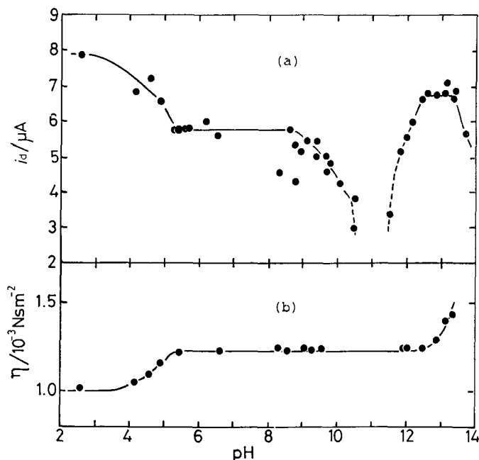
Fig. 3. Effects of pH on the diffusion current, i_d , of Pb(II) in the presence of 1 mol \text{dm}^{-3} \text{OAc}^- and their viscosity, \eta .
