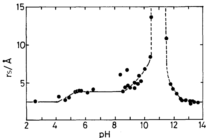
Fig. 4. Radii of Pb(II) complexes in the presence of 1 mol dm -3 with various pH values.
