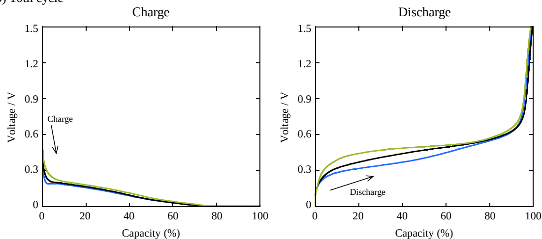
Fig. 8 Charge and discharge curves for the (a) 2nd and (b) 10th cycles of SiO/EC:DEC(1:1) + 1 mol L -1 LiPF 6 /Li cells in the voltage range of 0.005–1.5 V at 298 K. Charge conditions (2nd cycle): a constant current of 450 mA g -1 until a voltage of 0.005 V and a constant voltage of 0.005 V until a current of 15 mA g -1 . Charge conditions (after 3rd cycle): a constant current of 750 mA g -1 until a voltage of 0.005 V and a constant voltage of 0.005 V until a current of 15 mA g -1 . Discharge conditions (2nd cycle): a constant current of 450 mA g -1 until a voltage of 1.5 V. Discharge conditions (after 3rd cycle): a constant current of 750 mA g -1 until a voltage of 1.5 V.
