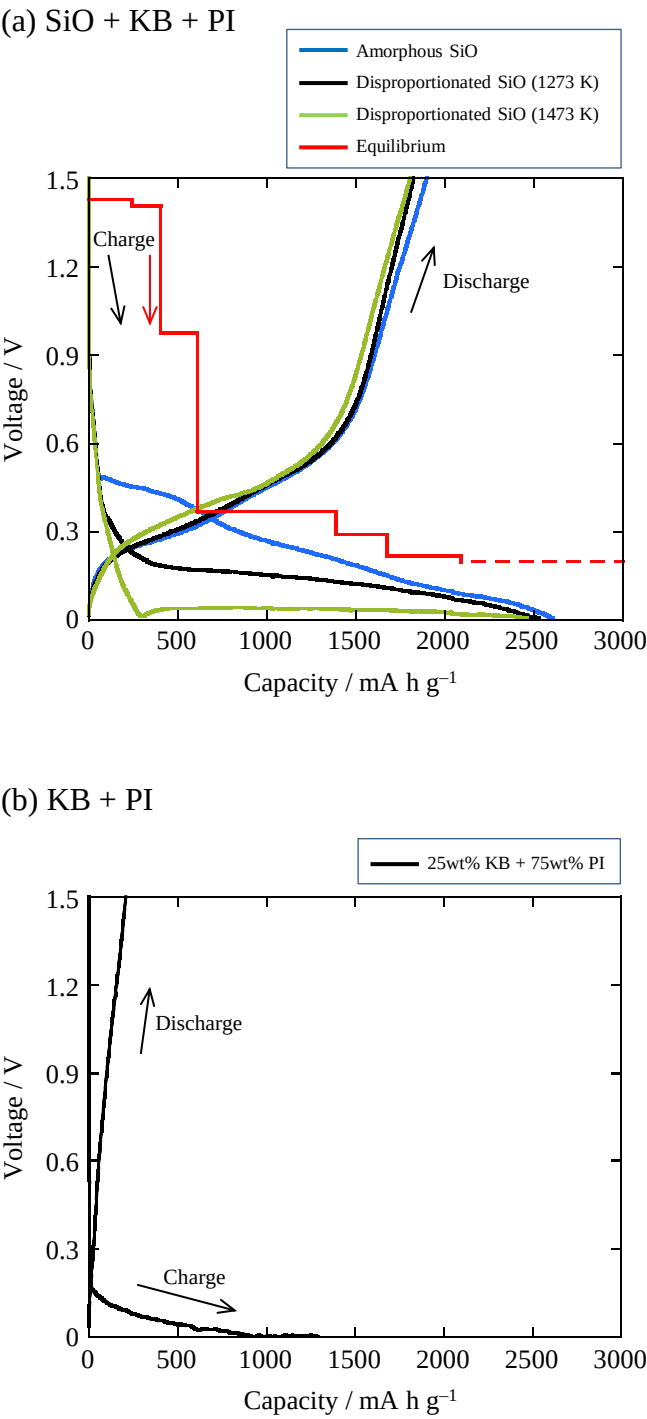
Fig. 5 (a) Charge and discharge curves for the 1st cycle of SiO/EC:DEC(1:1) + 1 mol L -1 LiPF 6 /Li cells in the voltage range of 0–1.5 V at 298 K. Charge conditions: a constant current of 15 mA g -1 until a voltage of 0 V. Discharge conditions: a constant current of 15 mA g -1 until a voltage of 1.5 V. (b) Charge and discharge curves for the 1st cycle of KB+PI/EC:DEC(1:1) + 1 mol L -1 LiPF 6 /Li cells in the voltage range of 0–1.5 V at 298 K. Charge conditions: a constant current of 10 mA g -1 until a voltage of 0 V. Discharge conditions: a constant current of 10 mA g -1 until a voltage of 1.5 V.
