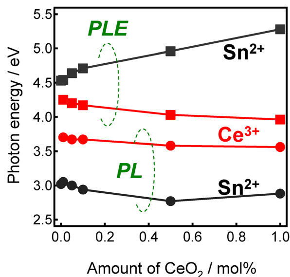
FIG. 4. Peak photon energies of x CeSZP glasses as a function of \text{CeO}_2 amount.
