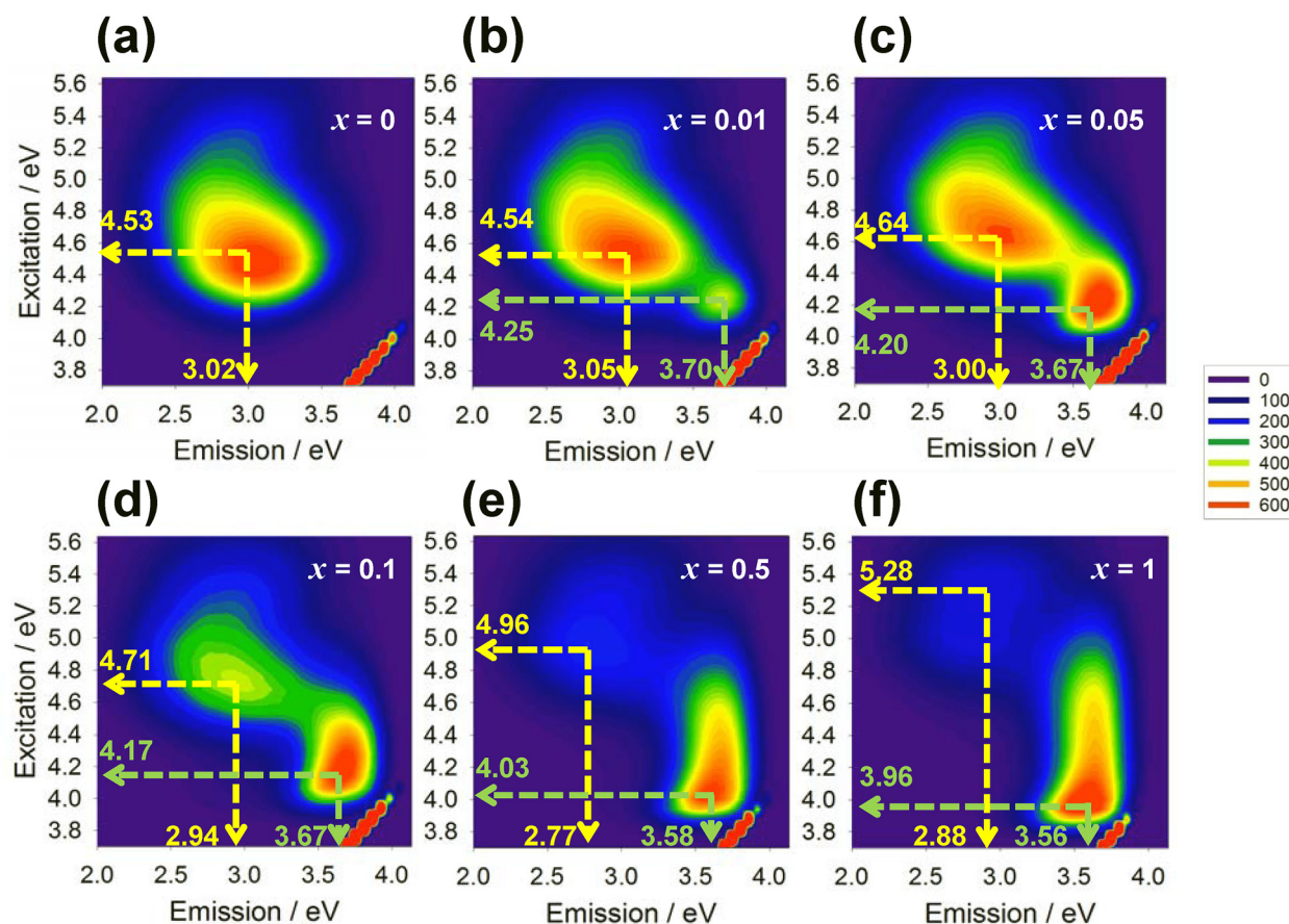
FIG. 3. Contour plots of PL intensity of the x CeSZP glasses with different amounts of Ce concentration. (a) 0, (b) 0.01, (c) 0.05, (d) 0.1, (e) 0.5, and (f) 1.0 mol. %. Linear scale is used for the intensity axis.
