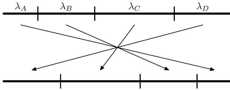
Figure 1: An interval exchange map
