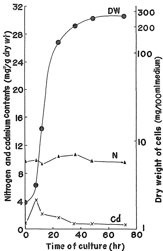
Fig. 7. Changes in cadmium and nitrogen contents of cells during the growth of resistant strain in 0.4 mM Cd-PGY medium. DW: Dry weight of cells; Cd: cadmium content; N: nitrogen content.
