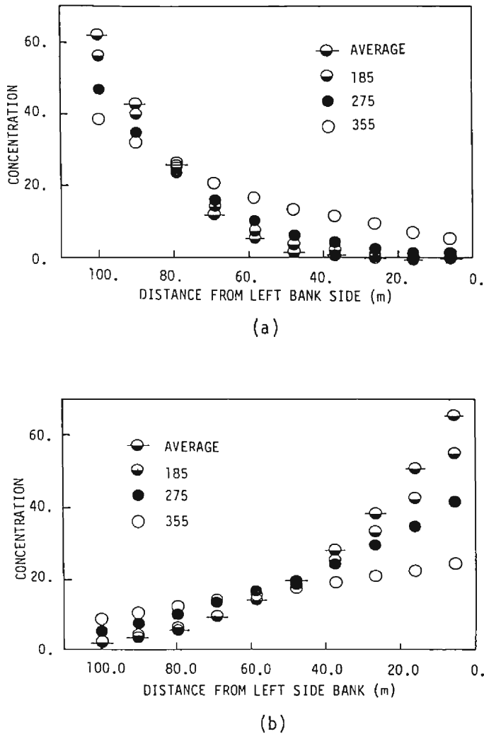
Fig. 19. Transverse distributions of concentration at 33.6km section simulated under the various flow regimes. (a) Tracer from the Katsura River, and (b) tracer from the Kizu River.
