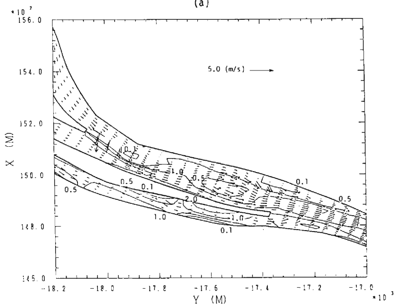
Fig. 9. Flow behavior and mixing at the confluence simulated in 61-1028 Test. (a) Momentum flux vector distributions and the iso-contour map of the bottom elevation, and (b) depth-averaged velocity vector distributions and the iso-contour lines of water depth.
