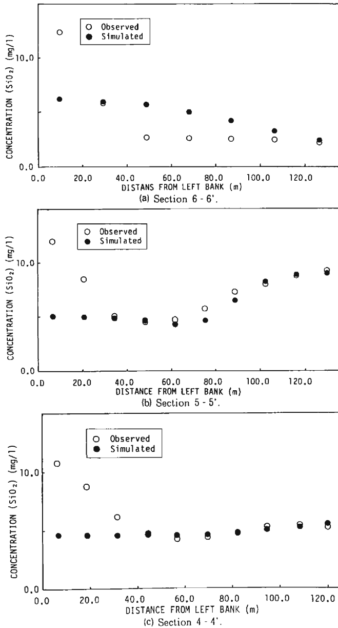
Fig. 13. Transverse distributions of \text{SiO}_2 concentration simulated in 61-1028 Test and measured ones. (a) 6-6' (34.8km) section, (b) 5-5' (34.2km) section, and (c) 4-4' (33.6km) section.
