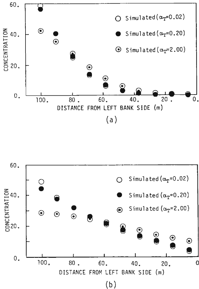
Fig. 22. Transverse distributions of tracer concentration from the Katsura River under various transverse mixing coefficients in ordinary (185-day) discharge condition for (a) 33.6km section, and (b) 32.08km section.
