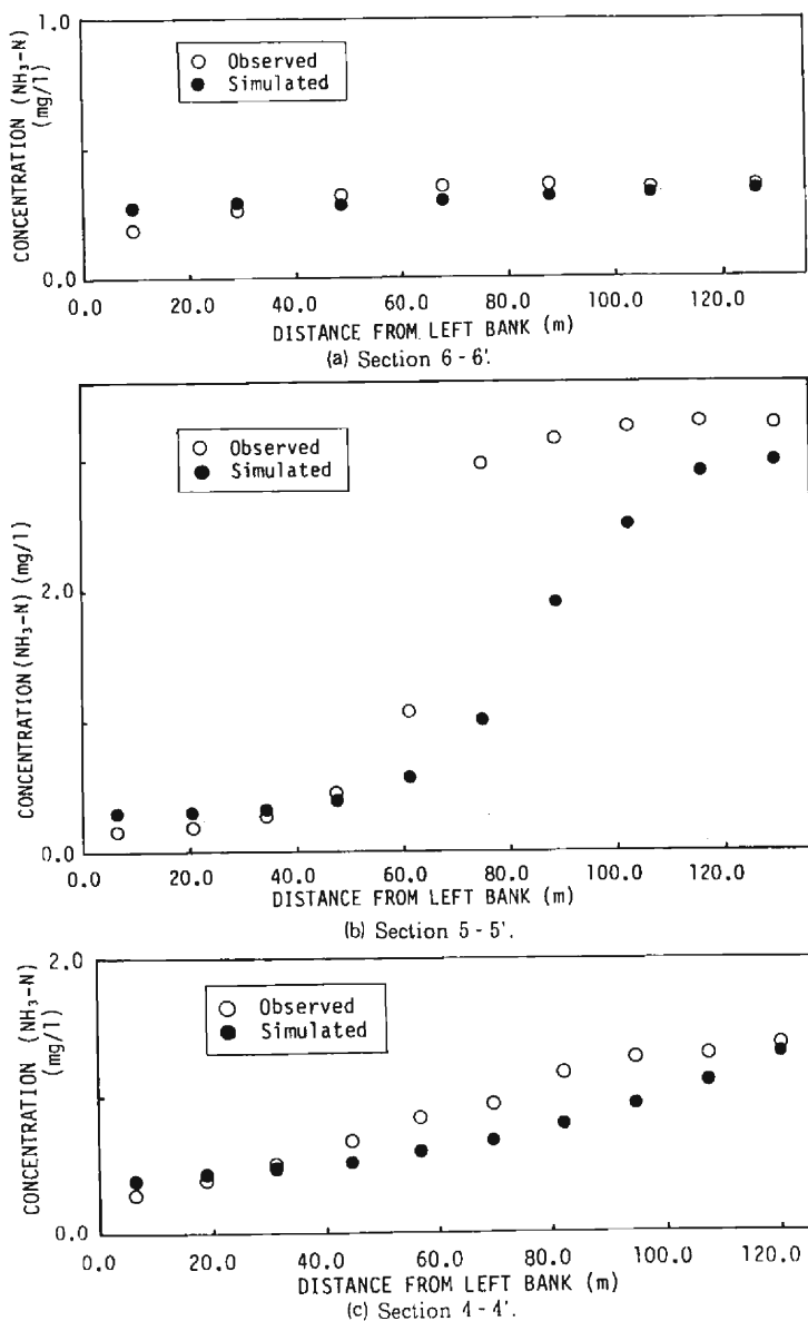
Fig. 12. Transverse distributions of \text{NH}_3\text{-N} concentration simulated in 61-1028 Test and measured ones. (a) 6-6' (34.8km) section, (b) 5-5' (34.2km) section, and (c) 4-4' (33.6km) section.
