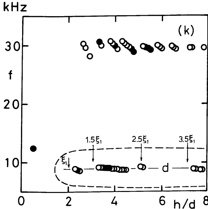
Fig. 4 Frequencies of discrete tone for small plate ( D/d = 0.35 ) as a function of nozzle-to-plate distance: (a) R = 2.26 , (b) R = 2.45 , (c) R = 2.93 , (d) R = 3.12 , (e) R = 3.32 , (f) R = 3.90 , (g) R = 4.29 , (h) R = 4.48 , (i) R = 4.68 , (j) R = 4.87 , (k) R = 5.84 .
