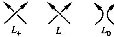
Fig. 5 Three knots L_+ , L_- and L_0
