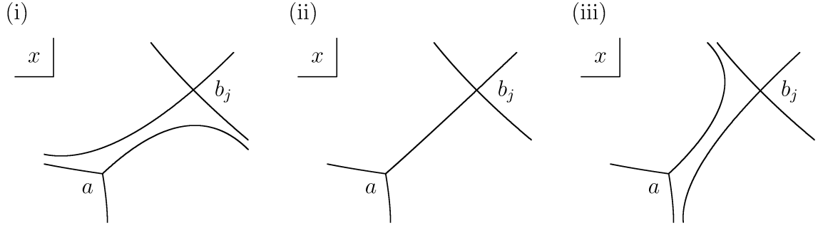
Figure 4 : Configuration of Stokes curves of (SL_I)_m when (i) t belongs to \Omega_1 , (ii) t lies in a Stokes curve and (iii) t belongs to \Omega_2 .
