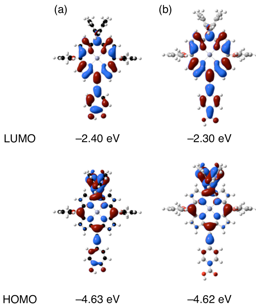
Figure S6. Selected molecular orbital diagrams for (a) YD2- o -C8T and (b) YD2- o -C8 obtained by DFT calculations with B3LYP/6-31G(d). To simplify the calculations, alkyl chains on the diarylamino groups were replaced with methyl ones, whereas octyloxy groups on the phenyl groups were replaced with methoxy ones.
