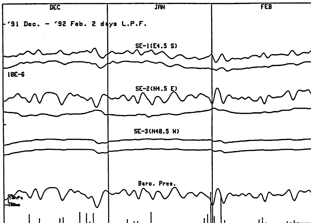
Fig. 5. Strain records of low pass filter for 2 day (upper part of each component) and strain changes removed it due to atmospheric pressure (lower).
