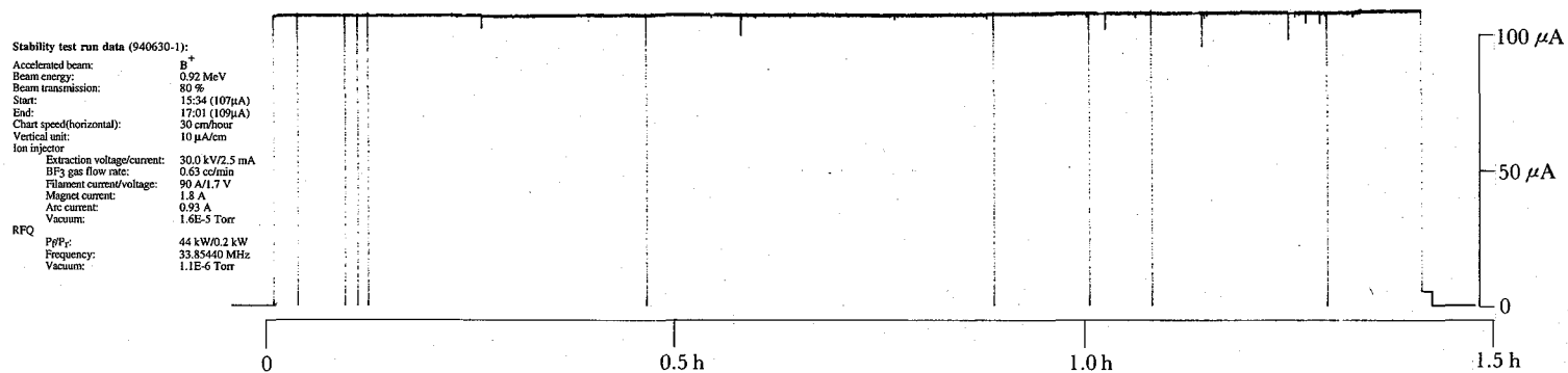
Fig. 6. B + beam stability test. The beam current is 100 μA at energy 0.92 MeV. The beam fluctuation is < \pm 1.0\%
