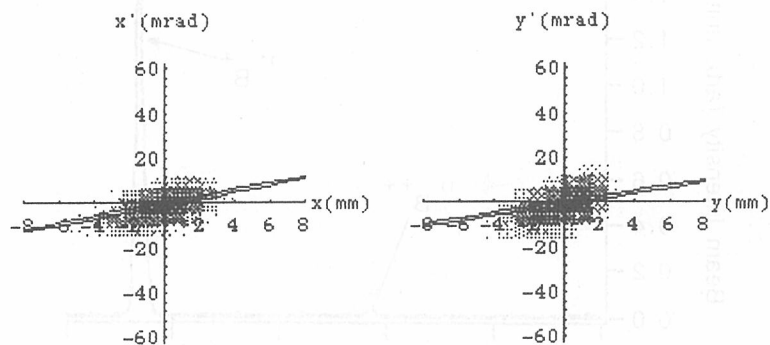
Fig. 5. \text{B}^+ emittance data for the input and output of the RFQ.
