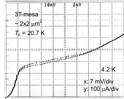
FIG. 3. The positive voltage part of the IV characteristics at 4.2 K for the 2 \times 2 \mu\text{m}^2 3T mesa in Fig. 2(b). The characteristics were observed by subtracting the Ohmic resistive component of 250 \Omega using a differential circuitry to remove influence of the contact resistance.
