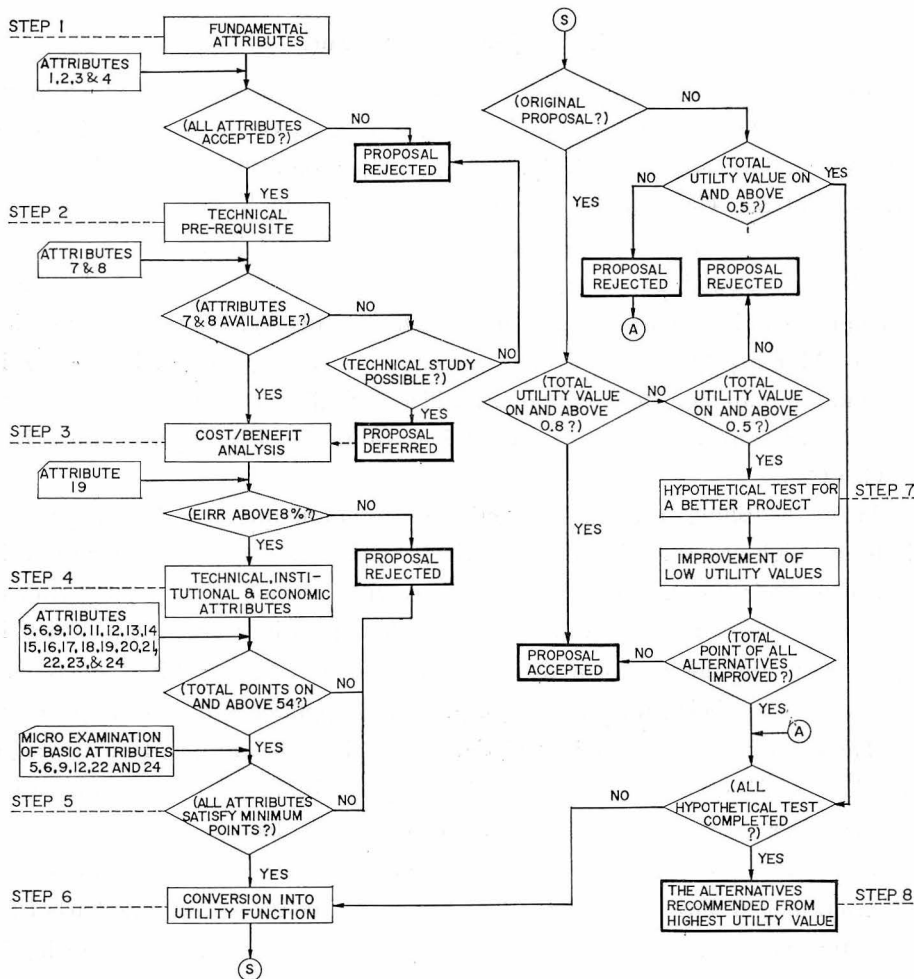
Fig. 1. Flow Chart of the Model (Approach to Overall Project Evaluation a Fishing Port Project)
