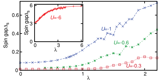
FIG. 5. (Color online) Spin gap \Delta_S , Eq. (5) as a function of \lambda for different U 's and fixed L . For small \lambda the gap is an increasing function of disorder as a consequence of the band structure of the quasiperiodic potential. Close to the insulator transition \lambda \lesssim \lambda_c , there is an additional gap enhancement caused by eigenfunction correlations [3].
