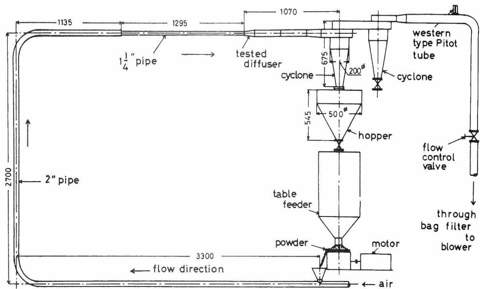
Fig.7.2 Schematic diagram of the experimental setup
