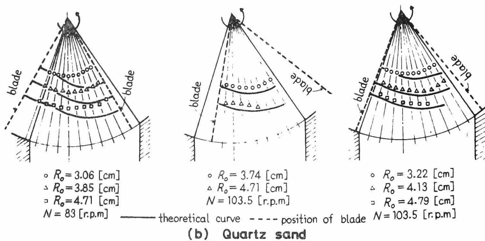
Fig.6.8 Particle trajectories
