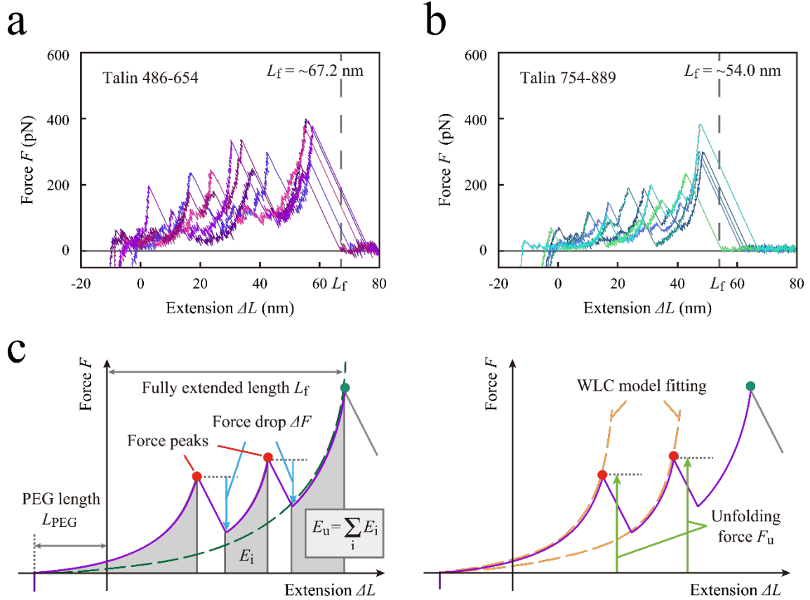
Fig. 2 Force curves for residues 486–654 and 754–889 of talin.
