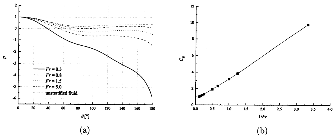
Fig. 14: (a) Pressure on the sphere surface. \theta is the angle measured from the lower stagnation point. (b) Froude number dependence of the drag coefficient of the sphere. Both figures are drawn for Re = 200 .
