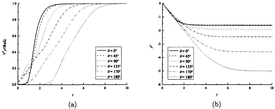
Fig. 9: (a) Time development of the density diffusion \nabla^2 \rho' / ReSc at selected six points on the sphere surface. (b) Time development of the density perturbation \rho' at selected six points on the sphere surface. In both figures, \theta is the angle measured from the lower stagnation point of the sphere. ( Fr = 0.3, Re = 200 ).
