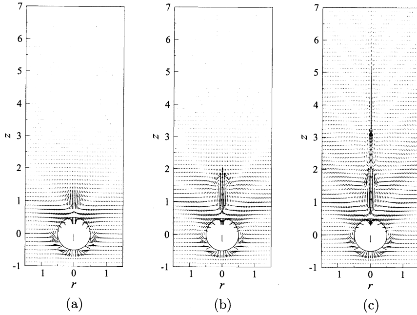
Fig. 8: Time development of velocity vector diagram in a stationary frame. (a) t = 0.5 , (b) t = 1.0 , (c) t = 10.0 .
