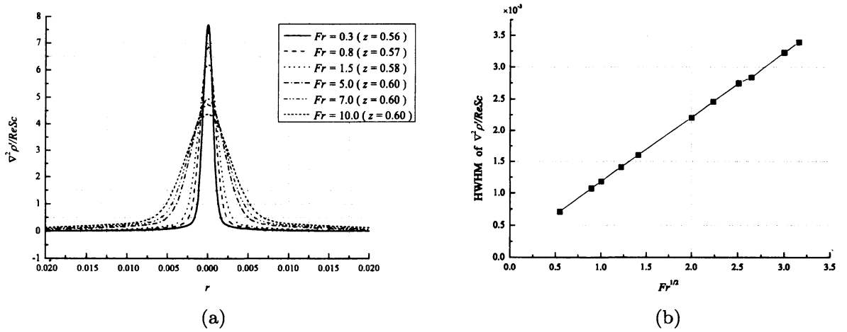
Fig. 12: (a)Froude number dependence of the steady state distribution of \nabla^2 \rho' / ReSc near the z axis at the height where \nabla^2 \rho' / ReSc becomes maximum. (b)Froude number dependence of the half width at half maximum (HWHM) of \nabla^2 \rho' / ReSc .
