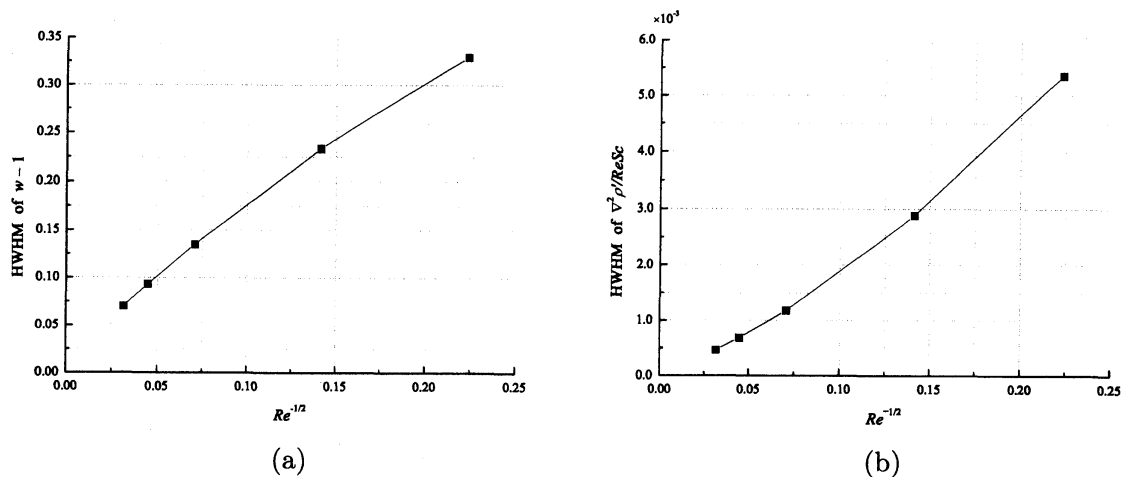
Fig. 13: Reynolds number dependence of HWHM of (a) w - 1 , (b) \nabla^2 \rho' / Re Sc .
