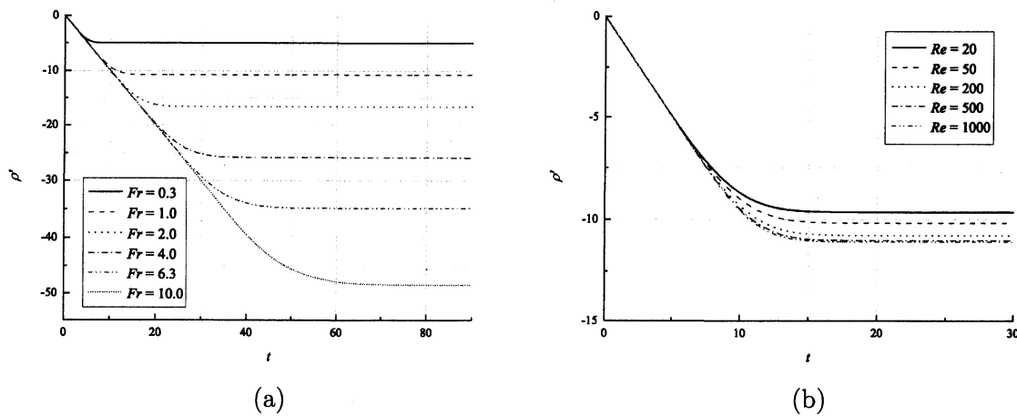
Fig. 10: Time development of the density perturbation \rho' at the upper stagnation point of the sphere ( \theta = 180^\circ ). (a) Froude number dependence ( Re = 200 ), (b) Reynolds number dependence ( Fr = 1 ).
