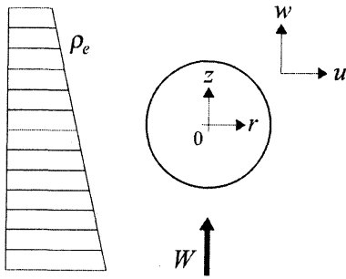
Fig. 2: Schematic figure of a sphere moving downward in a stratified fluid. A frame moving vertically downward with the sphere is used, and the linearly stratified fluid moves up at a constant speed W relative to the sphere.
