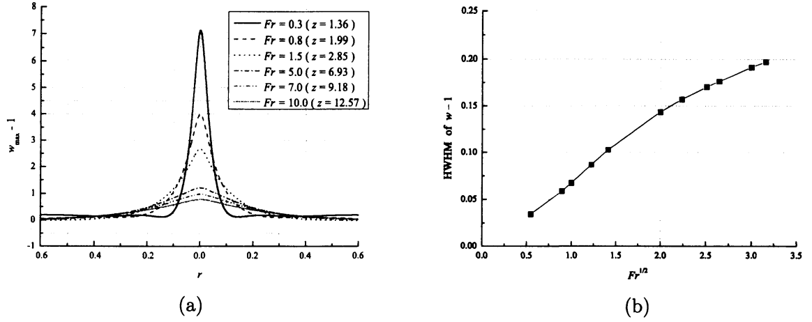
Fig. 11: (a)Froude number dependence of the steady state distribution of the vertical velocity w - 1 near the z axis at the height where w becomes maximum. (b)Froude number dependence of the half width at half maximum (HWHM) of w - 1 .
