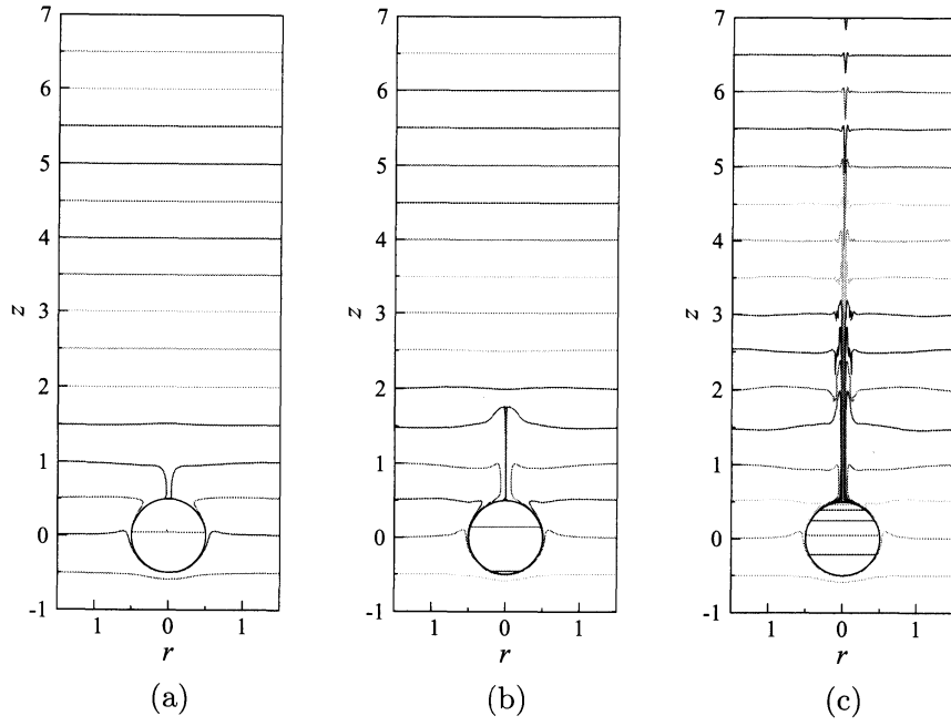
Fig. 7: Time development of the isopycnal lines of total density \rho ( Fr = 0.3, Re = 200 ). The lines drawn in the circle represent the density distribution on the sphere surface. Contour interval \Delta\rho = 0.5 . (a) t = 0.5 , (b) t = 1.0 , (c) t = 10.0 .
