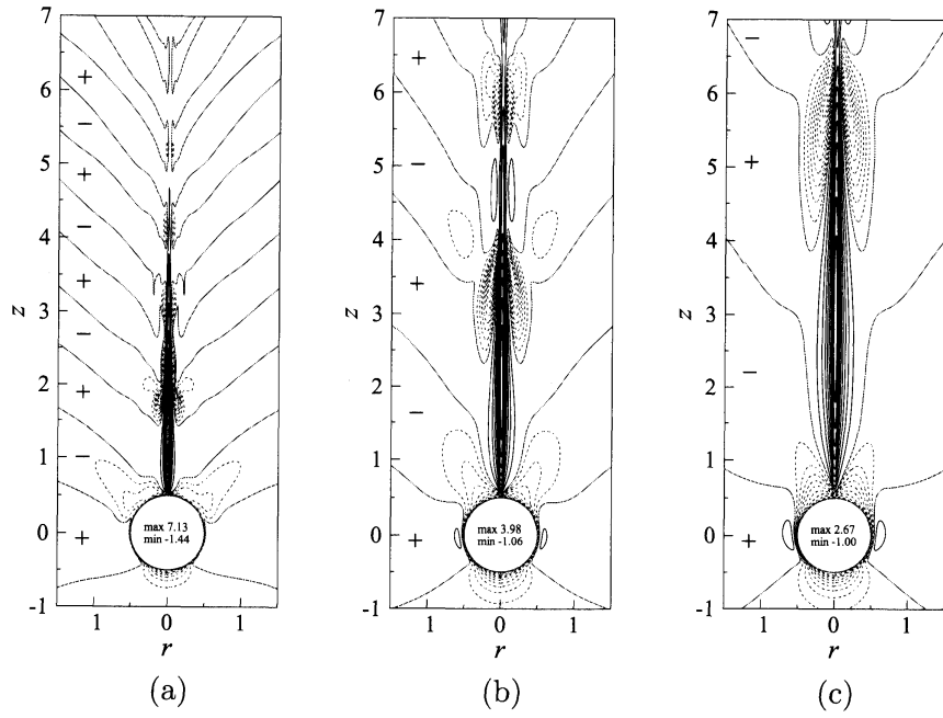
Fig. 5: Contours of vertical velocity in stationary frame, i.e. w - 1 , at t = 30 . The interval of \Delta(w - 1) = (w_{\max} - 1)/10 for w - 1 > 0 (solid lines), and |w_{\min} - 1|/10 for w - 1 < 0 (dashed lines). Broad lines represent w - 1 = 0 . (a) Fr = 0.3 , (b) Fr = 0.8 , (c) Fr = 1.5 .
