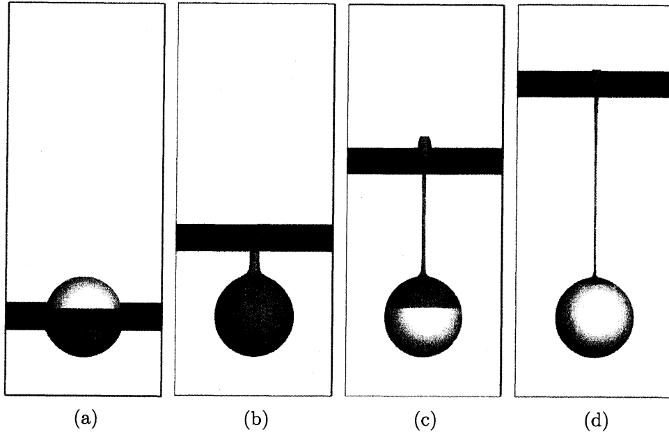
Fig. 6: Typical deformation process of an isopycnal surface ( Fr = 0.3 , Re = 200 ). The surface is initially located at z = -1 as a horizontal plane. (a) t = 1.0 , (b) t = 2.0 , (c) t = 3.0 , (d) t = 4.0 .
