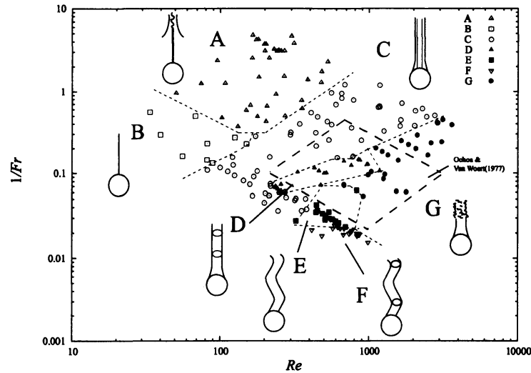
Fig. 1: Classification of the wake structures with Fr and Re . From Hanazaki, Kashimoto & Okamura (2009).
