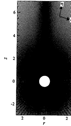
Fig. 3: Computational grid near the sphere. Every two grid line is drawn.
