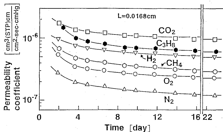
Fig. 6. Effect of thermal hysteresis on gas permeability of poly(TMSP-co-PP) (9:1) membrane at 30°C. Heat treatment was carried out at 75°C under vacuum between measurements.
