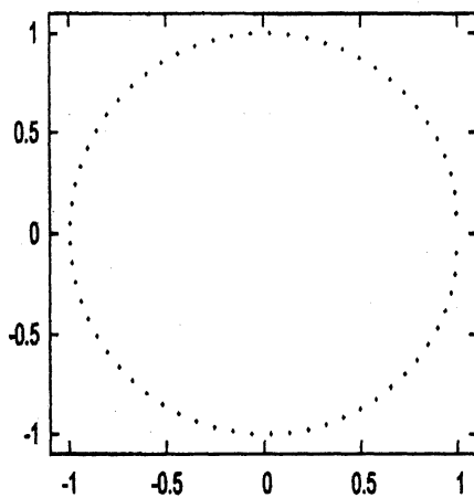
图 10. Roots of P_m = 0 ( m = 256 ).
