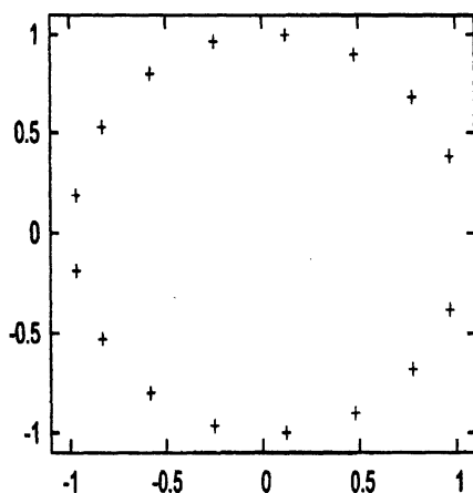
図 6. Roots of P_m = 0 ( m = 16 ).
