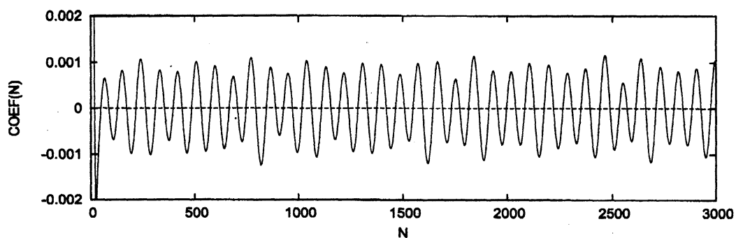
图 4: Coefficients of the Taylor series of F'(t)/F(t) ; NMX=3000 .
