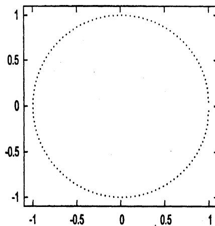
图 11. Roots of P_m = 0 ( m = 512 ).
