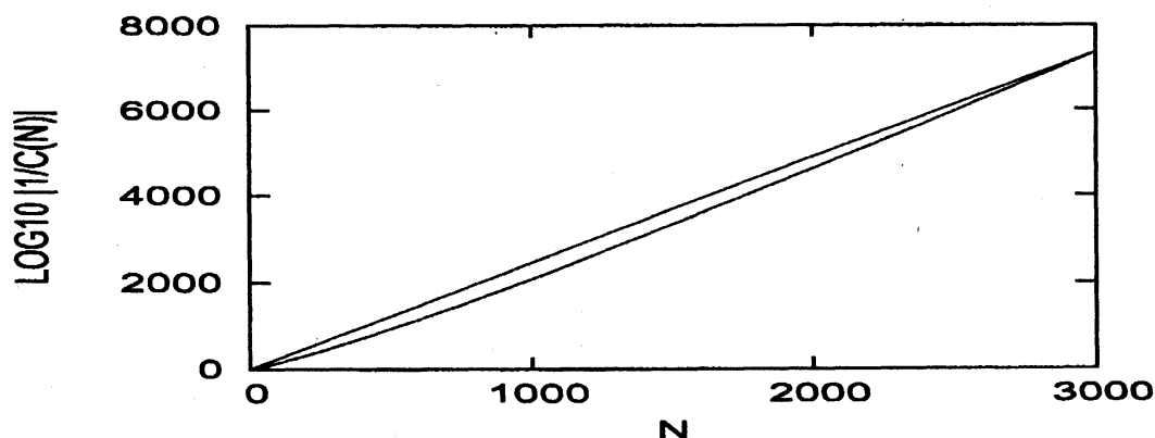
図 1: \log_{10} |1/c(n)| , for n = 0, \dots, 3000
