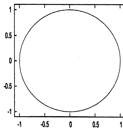
图 13. Roots of P_m = 0 ( m = 2048 ).
