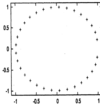
図 7. Roots of P_m = 0 ( m = 32 ).
