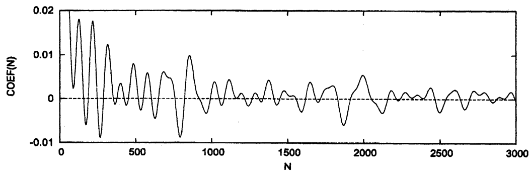
图 5: Coefficients of the Taylor series of \log F(t) ; NMX=3000 .
