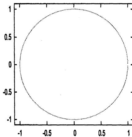
图 12. Roots of P_m = 0 ( m = 1024 ).
