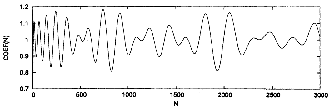
图 3: Coefficients of the Taylor series of 1/F(t) ; NMX=3000 .
