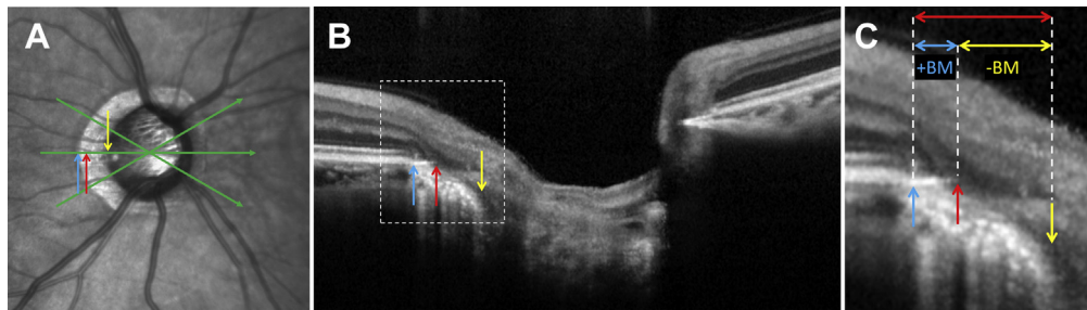
Figure 1. Microstructure of \beta -zone peripapillary atrophy (PPA). A , Infrared (IR) fundus image of the optic disc. The 3 green arrowed lines indicate the scanned locations centered on the optic disc. The 3 B-scans comprise horizontal and upper and lower scans, defined as scans 30^\circ above and below the horizontal scan, respectively. B , Spectral-domain optical coherence tomography (SD OCT) B-scan image of the location indicated by horizontal green arrowed line in A . C , Magnified image of the rectangular area indicated by broken white lines in B . The blue, red, and yellow arrows in A , B , and C indicate \beta -zone PPA margin, Bruch's membrane (BM) opening, and optic disc margin, respectively. The red, blue, and yellow 2-directional arrows in C show \beta -zone PPA width, \beta -zone PPA with BM ( PPA_{+BM} ) width, and \beta -zone PPA without BM ( PPA_{-BM} ) width, respectively.
