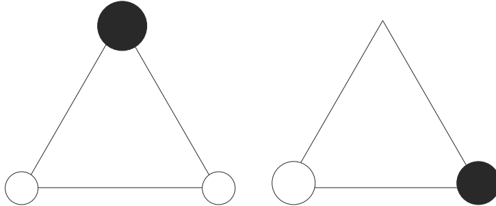
Figure 1.2: Symmetry adapted molecular orbitals of the triangle molecule.
