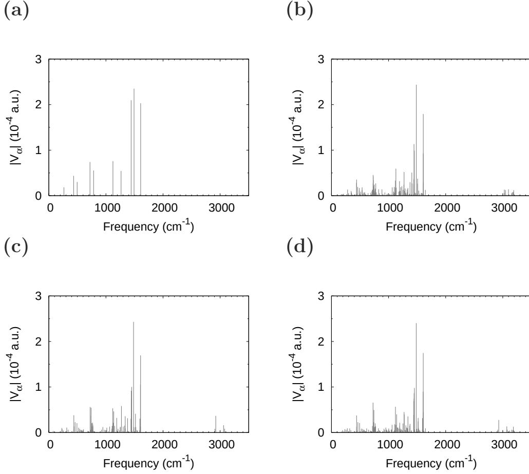
Figure 4.2: Vibronic coupling constants of (a) C_{60}^- , (b) PCBM^- , (c) C_{60} pyrrolidine ^- ( C_s ), and (d) C_{60} pyrrolidine derivative ^- ( C_1 ) in 10^{-4} a.u.
