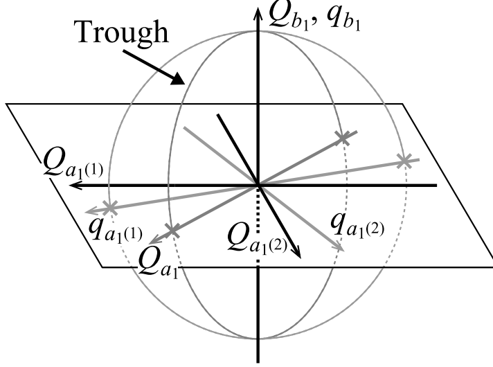
Figure 2.1: Mass-weighted normal coordinates (Q_{a_1(1)}, Q_{a_1(2)}, Q_{b_1}) , effective coordinates (q_{a_1(1)}, q_{a_1(2)}, q_{b_1}) , and the trough.
