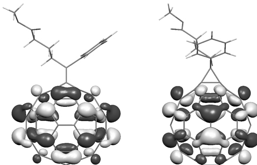
(b) \Delta\rho
