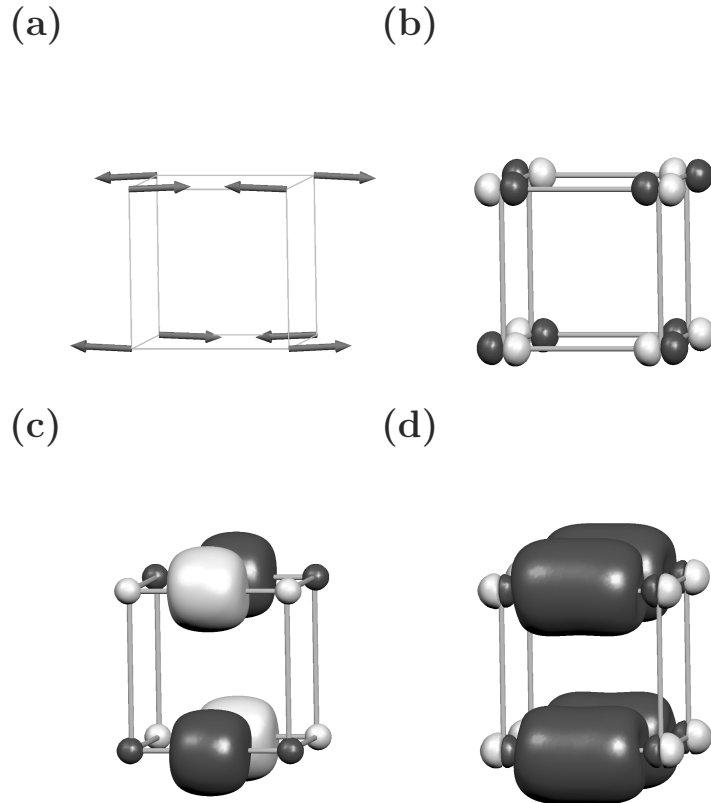
Figure 1.6: Vibronic coupling density analysis for t_{2g}(2) mode of \text{Li}_8^+ . (a) t_{2g}(2) mode, (b) potential derivative v(\mathbf{r}) (isovalue: 1.0 \times 10^{-2} a.u.), (c) overlap density \rho_{x,y}(\mathbf{r}) (isovalue: 1.0 \times 10^{-3} a.u.), and (d) VCD \eta(\mathbf{r}) (isovalue: 1.0 \times 10^{-6} a.u.).
