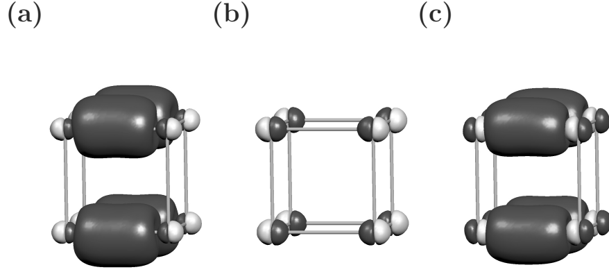
Figure 1.5: Vibronic coupling density for t_{2g}(2) mode of \text{Li}_8^+ (isovalue: 1.0 \times 10^{-6} a.u.). (a) VCD \eta(\mathbf{r}) , (b) zero component \eta'(\mathbf{r}) , and (c) RVCD \bar{\eta}(\mathbf{r}) . Light grey is positive, and dark gray is negative.
