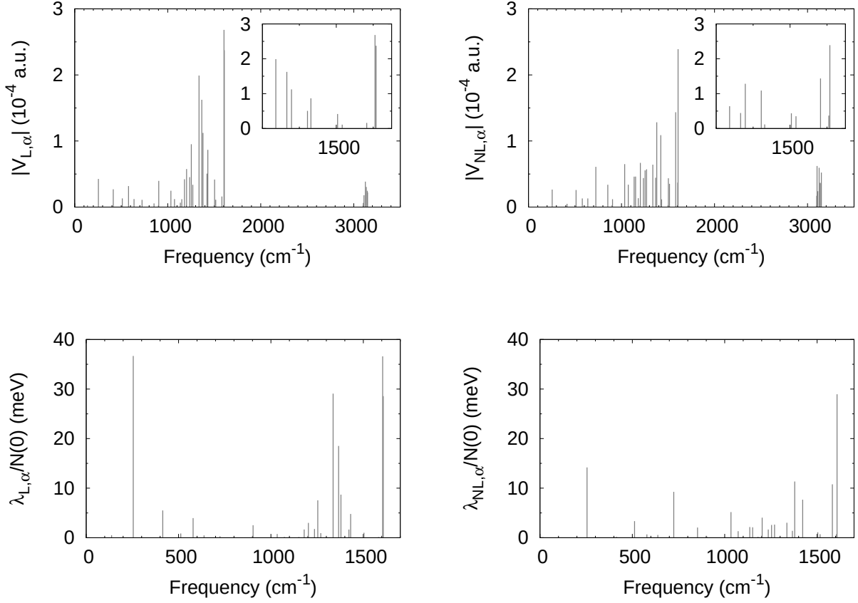
Figure 3.2: Calculated (top) orbital vibronic coupling constants V_{i,\alpha} and (bottom) electron-phonon couplings \lambda_{i,\alpha}/N(0) in the (a) monoanion and the (b) trianion. The subscripts L and NL denote LUMO and NLUMO, respectively. Insets show the orbital vibronic couplings between 1300 to 1650 \text{cm}^{-1} .
