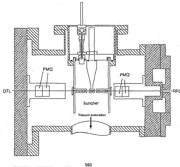
Fig. 4. The RF phase buncher.
