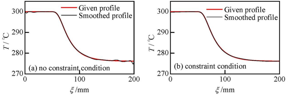
Figure 13 Comparison of the given temperature profile (exact solution) after smoothing with the noisy profile: (a) without and (b) with constraint conditions
