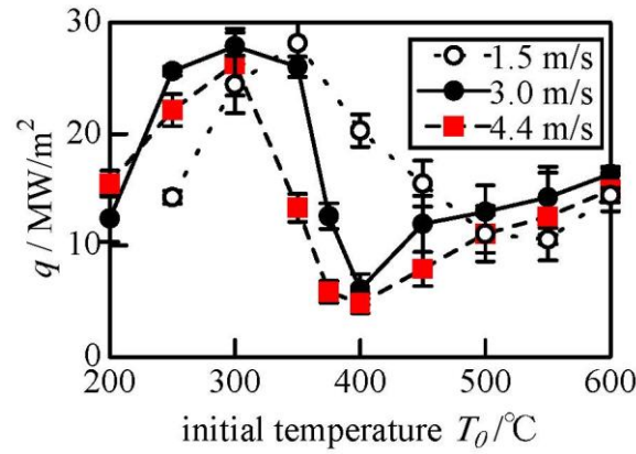
Figure 17 Maximum heat flux under various conditions for H = 0.5 mm and Q = 6.35 L/min.
