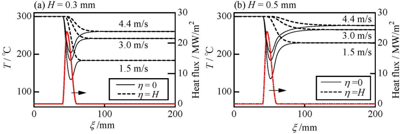
Figure 4 Exact solutions for varying velocity of solid ( V_s = 1.5, 3.0 , and 4.4 m/s) and H = (a) 0.3 ; and (b) 0.5 mm
