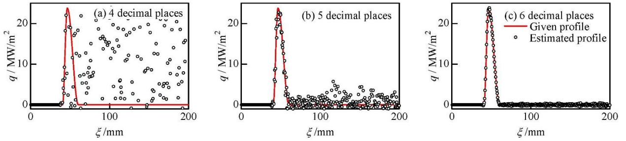
Figure 11 Heat-flux profiles on the cooled surface evaluated using the temperature rounded off from the exact solution to 4–6 decimal places for the case of H = 0.5 mm and V_s = 4.4 m/s
