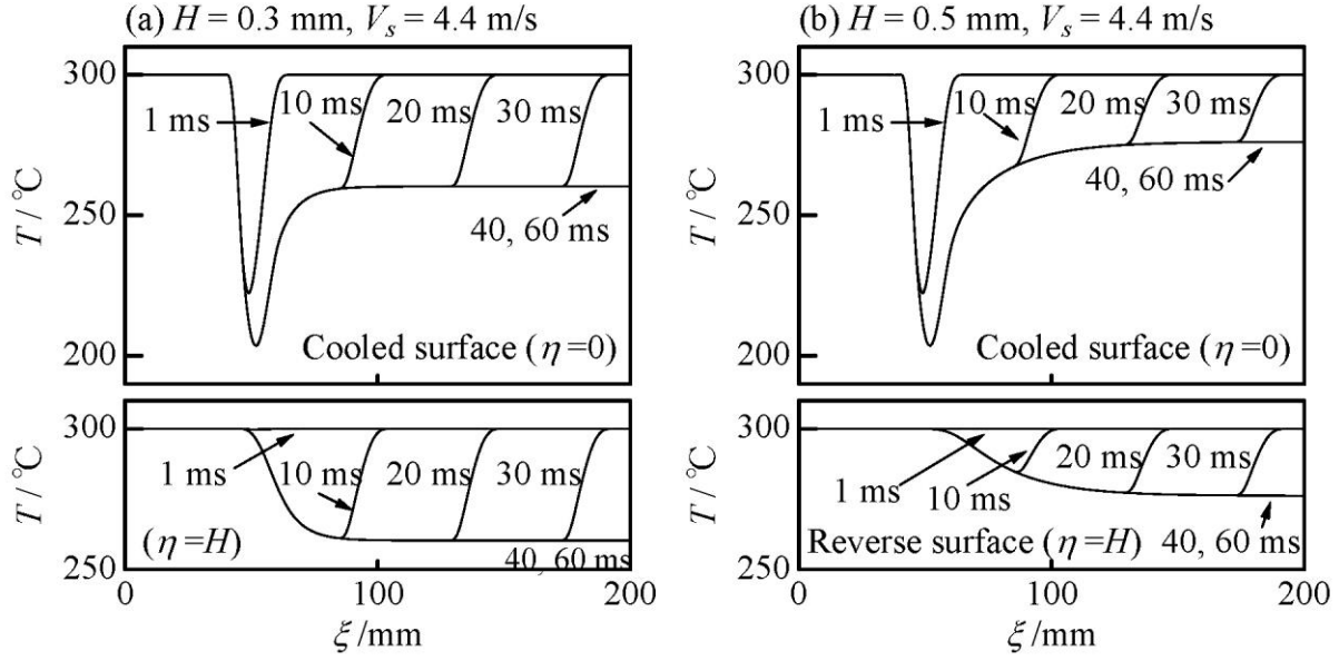
Figure 3 Examples of transient temperature profiles inside the cooled and reverse surfaces, calculated using the exact solution of Eq. 5 for: V_s = 4.4 m/s, t = 0 –60 ms, and H = (a) 0.3 and (b) 0.5 mm
