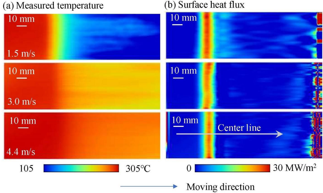
Figure 16 Temperature profile of (a) the uncooled surface and (b) estimated heat flux distribution for T_0 = 300\text{ }^{\circ}\text{C} , H = 0.5\text{ mm} , and Q = 6.35\text{ L/min} .
