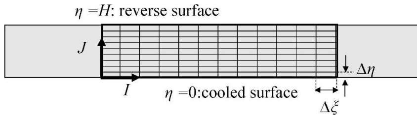
Figure 6 Overview of computational domain
