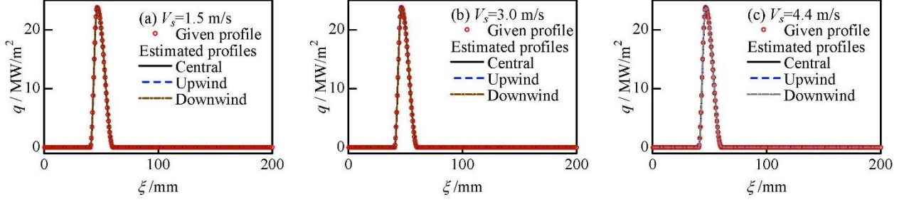
Figure 8 Comparisons of the given heat flux with model predictions for H = 0.3 mm and V_s = (a) 1.5, (b) 3.0, and (c) 4.4 m/s
