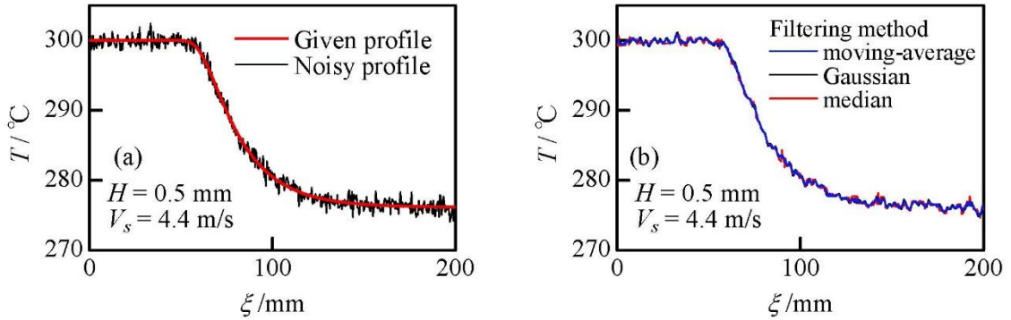
Figure 12 (a) Artificial temperature profile, Y , on the reverse surface for H = 0.5 mm and V_s = 4.4 m/s, and (b) temperature profiles obtained using various digital filtering methods.
