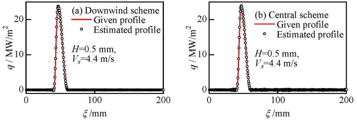
Figure 10 Comparison of the given heat flux and model predictions for H = 0.5 mm and V_s = 4.4 m/s, when (a) \varepsilon = \infty and (b) \varepsilon = -1
