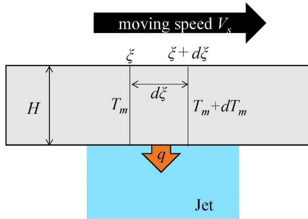
Figure 5 Schematic of the simple model
