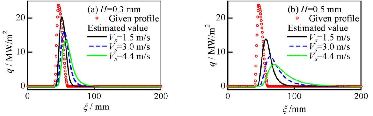
Figure 7 Validations of simple model by comparing the predictions with the given profile for: H = (a) 0.3 and (b) 0.5 mm; V_s = 1.5, 3.0, and 4.4 m/s
