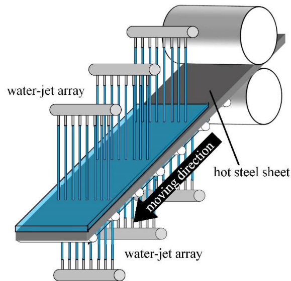
Figure 1 Schematic of run-out table cooling
