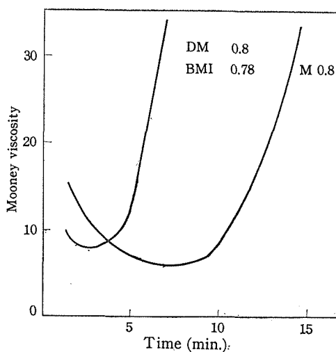
Fig. 3. Comparision of scorch between M compound and DM+BMI compound.
