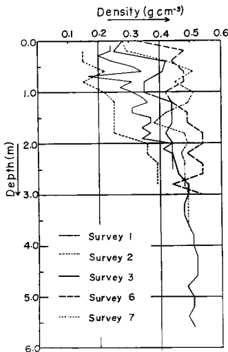
Fig. 2. (a) Density profile in snow layer.
