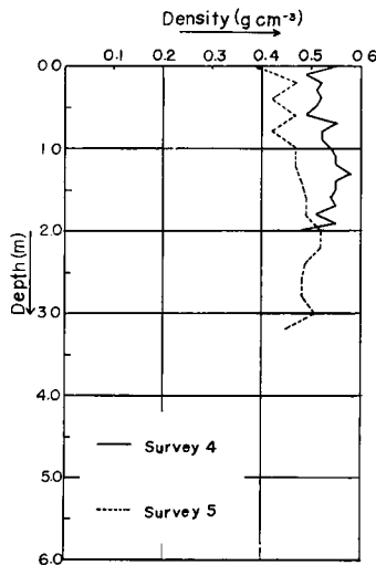
Fig. 2. (b) Density profile in snow layer.
