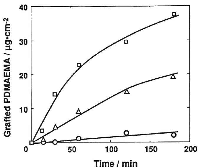
Fig. 2. Effect of UV irradiation time and monomer concentration on the yield of grafted PDMAEMA. [monomer] / wt %: (○) 0.1, (△) 1, (□) 3
