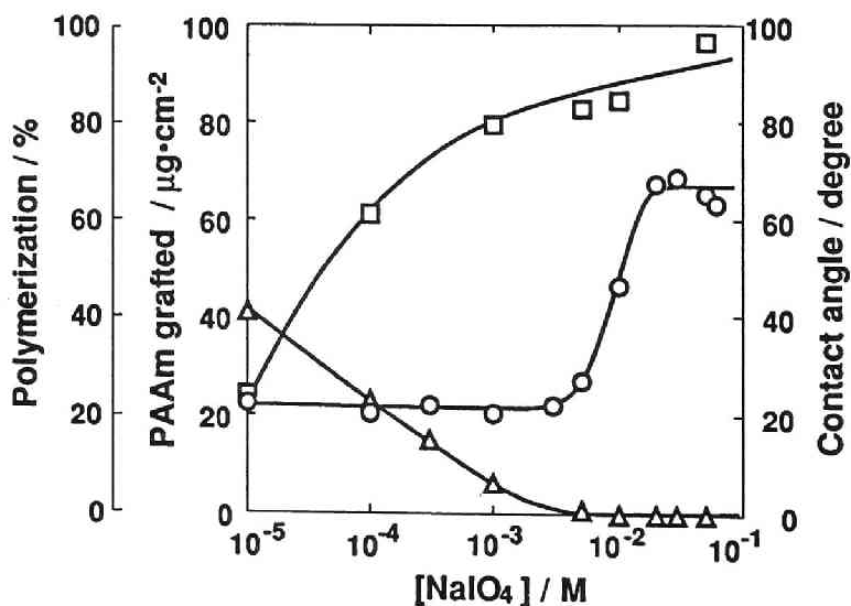
Fig. 4. AAm graft polymerization onto PET films under degassing by UV irradiation with \text{NaIO}_4 (10 wt % AAm, 35 °C, 90 min) : (□) total polymerization, (Δ) graft polymerization, (O) contact angle.
