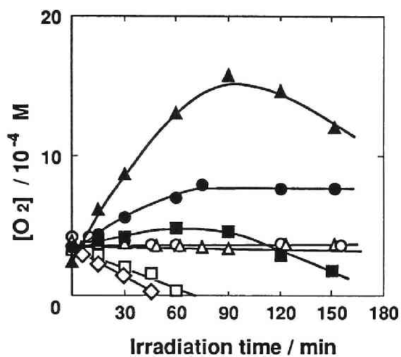
Fig. 7. UV irradiation effect on O 2 concentration of 10 wt % AAm solution containing NaIO 4 of different concentrations. [NaIO 4 ] / M: (○) 0, (△) 1x10 -4 , (□) 5x10 -4 , (◇) 1x10 -3 , (■) 1x10 -2 , (▲) 5x10 -2 , (●) 1x10 -3 (without AAm).
