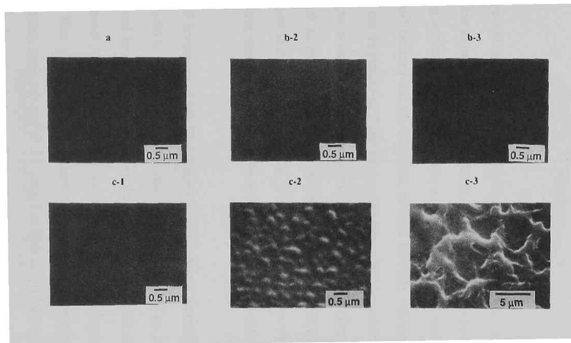
Fig.11. SEM photographs of grafted surfaces. a: virgin film, b: grafted film without complexation, c: grafted and ion complexed Mw of graft chain: (-1) 2.2 \times 10^4 , (-2) 5.3 \times 10^4 , (-3) 1.5 \times 10^5
