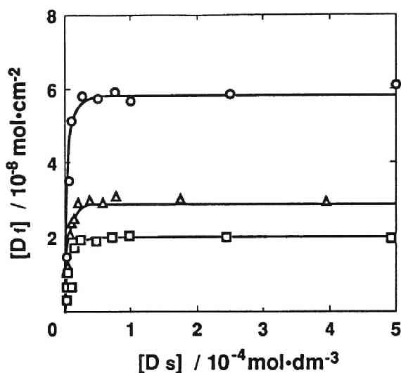
Fig. 6. Sorption isotherms of different anions on a DMAEMA-grafted PET film ( 9 \mu\text{g}\cdot\text{cm}^{-2} ) at pH 3 and 30^\circ\text{C} for 1h: (○) mono-SO 3 , (Δ) di-SO 3 , (□) tri-SO 3 .
