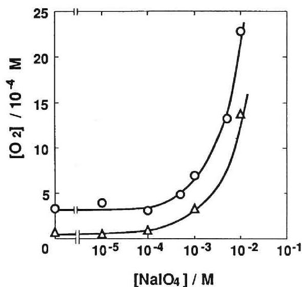
Fig.5 Change of O 2 concentration of NaIO 4 aqueous solution during UV irradiation (35 °C, 90 min): (O) without degassing, (Δ) with degassing.
