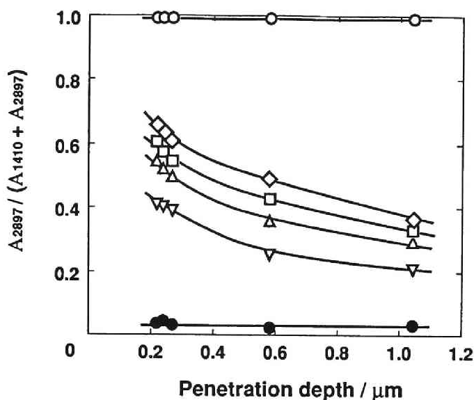
Fig. 9. The relative absorption by methylene group as a function of the penetration depth for grafted PET films. (●) virgin, (▽) grafted to 4 \mu\text{g}\cdot\text{cm}^{-2} , (Δ) grafted to 8 \mu\text{g}\cdot\text{cm}^{-2} , (□) grafted to 12 \mu\text{g}\cdot\text{cm}^{-2} , (◇) grafted to 20 \mu\text{g}\cdot\text{cm}^{-2} , (○) PEM-4 homopolymer
