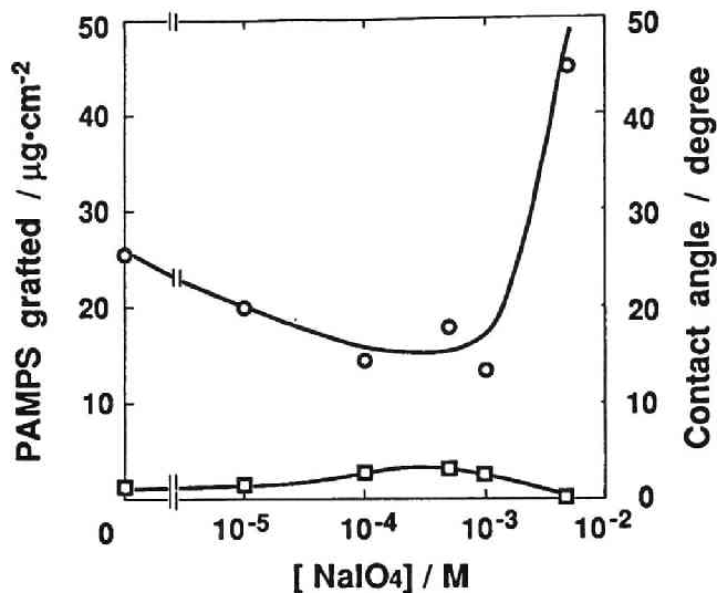
Fig. 2. Effects of NaIO 4 concentration on the graft polymerization of AMPS onto the PET film surface (10 wt % AMPS, 30 °C, 90 min). (O) contact angle, (□) density of PAMPS grafted
