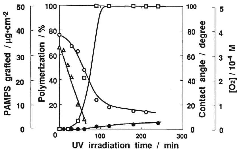
Fig. 3. Effects of irradiation time on the graft polymerization of AMPS onto the PET film surface (10 wt % AMPS, 5 \times 10^{-4} M \text{NaIO}_4 , 30 °C). (○) contact angle, (□) polymerization, (Δ) \text{O}_2 concentration, (●) density of PAMPS grafted
