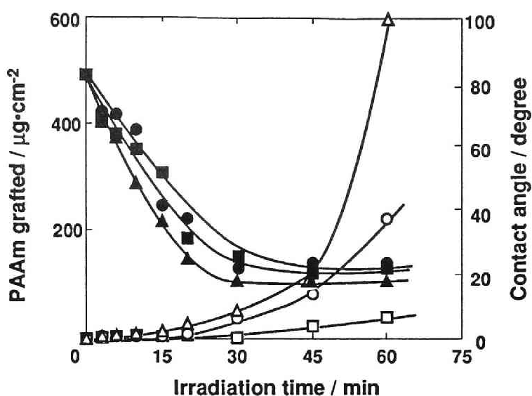
Fig. 5. Effect of temperature at UV irradiation of PET films pretreated with benzyl alcohol (30 min, 135°C, 3 atm): ( \square , \blacksquare ) 20°C, ( \circ , \bullet ) 35°C, ( \triangle , \blacktriangle ) 60°C. Open marks: graft amount, closed marks: contact angle.
