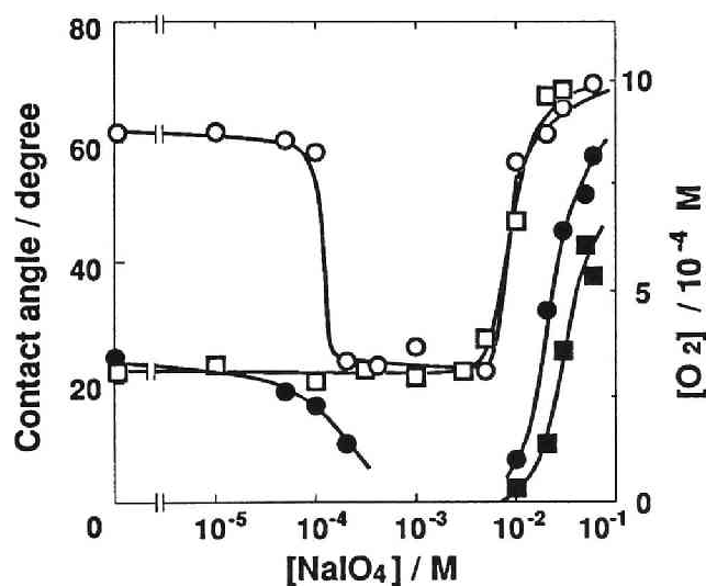
Fig. 6. Change of O 2 concentration of AAm solution containing NaIO 4 of different concentrations during UV irradiation (10 wt % AAm, 35°C, 90 min): (O, ●) without degassing, (□, ■) under degassing. Open marks: contact angle, closed marks: O 2 concentration.
