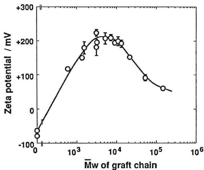
Fig. 6. Effect of the molecular weight of graft chain on the zeta potential of grafted film surface at pH 5 ( \text{KCl}=1 \times 10^{-3} \text{ M} ).
