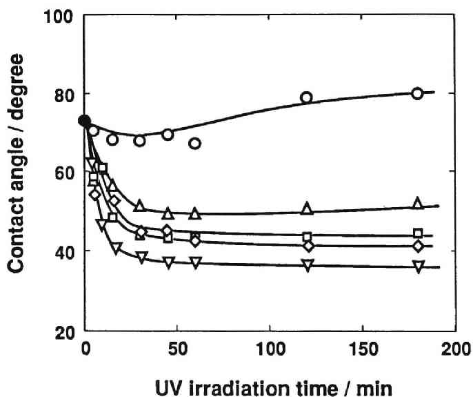
Fig. 3. Water contact angles of PET films grafted with PEM as a function of UV irradiation time (2.5 wt % PEM, 5x10 -4 M NaIO 4 , 30 °C). (●) virgin PET, (○) PEM-2, (Δ) -4, (□) -8, (◇) -22, (▽) -90
