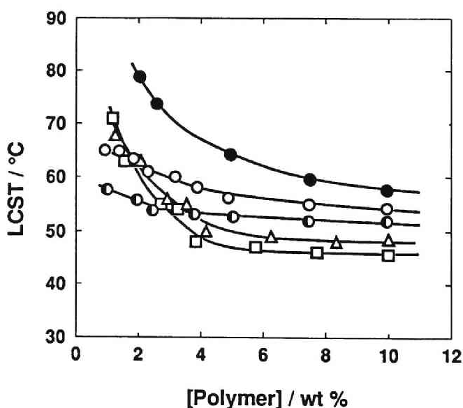
Fig. 4. Lower critical solution temperature (LCST) of PDMAEMA. \overline{M}_w : (○, ●, ○) 1.2 \times 10^5 , (△) 2.0 \times 10^5 , (□) 2.4 \times 10^5 (●) 1 \times 10^{-2} M HCl added, (○) 1 \times 10^{-3} M NaOH added, (○, △, □) without addition.
