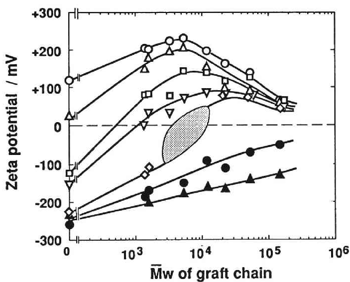
Fig. 7. Effect of pH on the zeta potential of film surfaces grafted with PDMAEMA of different molecular weights ( \text{KCl}=1 \times 10^{-3} \text{ M} ). pH: (O) 4.0, (Δ) 5.0, (□) 6.6, (▽) 7.0, (◇) 8.3, (●) 9.5, (▲) 10.5
