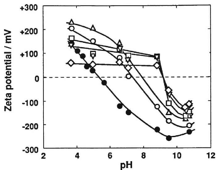
Fig. 8. Effect of pH on the zeta potential of films grafted with PDMAEMA of different molecular weights. \overline{MW} : (●) 0 (virgin PET film), (○) 2.2 \times 10^3 , ( \Delta ) 4.4 \times 10^3 , ( \square ) 2.2 \times 10^4 , ( \nabla ) 5.3 \times 10^4 , ( \diamond ) 1.5 \times 10^5
