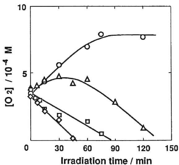
Fig. 8. UV irradiation effect on O 2 concentration of solution containing AAm of different concentrations and 1x10 -3 M NaIO 4 . [AAm] / wt %: (○) 0, (△) 5, (□) 7.5, (◇) 10.
