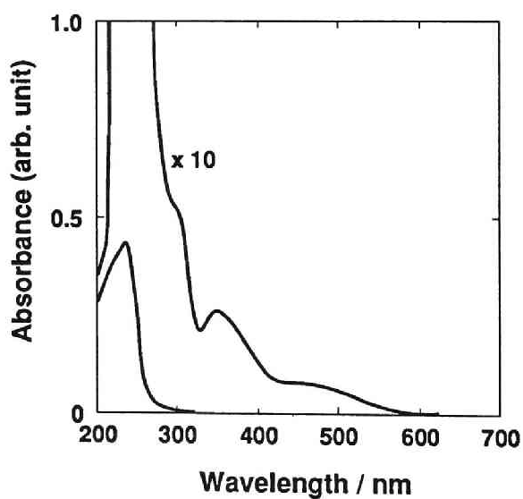
Fig. 10. Absorption spectra of 10 wt % aqueous AAm solution containing 5 \times 10^{-2} \text{ M} \text{NaIO}_4 irradiated with UV radiation for 12 h at 35^\circ \text{C} .
