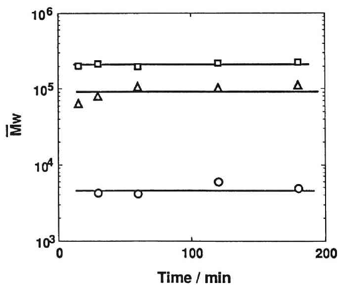
Fig. 3. Effect of UV irradiation time on the molecular weight of DMAEMA homopolymer. [monomer] / wt %: (○) 0.1, (△) 1, (□) 3
