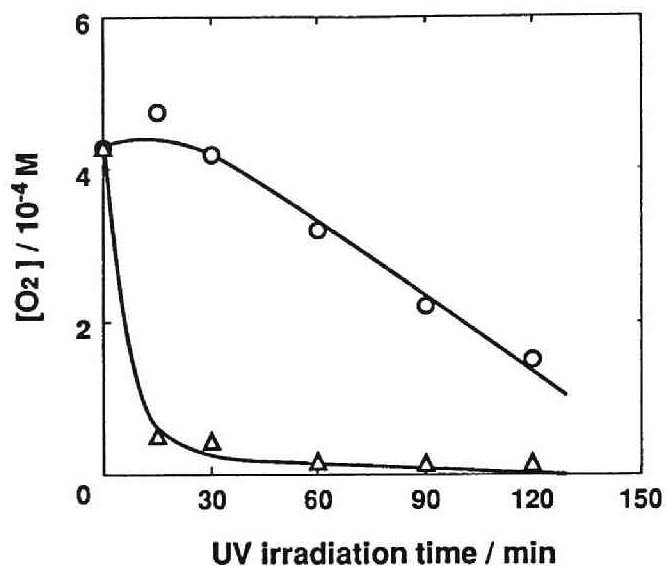
Fig. 2. Effect of the NaIO 4 addition on the consumption of O 2 in 10 wt % PEM-8 solution at 30 °C under UV irradiation. (O) without NaIO 4 , (Δ) with 5x10 -4 M NaIO 4 .
