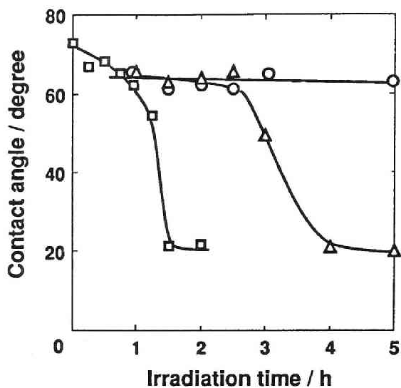
Fig. 3. Contact angles of PET films grafted with AAm without degassing at different \text{NaIO}_4 concentration by UV irradiation (10 wt % AAm, 35°C). [\text{NaIO}_4] / \text{M} : (O) 1 \times 10^{-4} , (□) 5 \times 10^{-3} , (Δ) 3 \times 10^{-2} .
