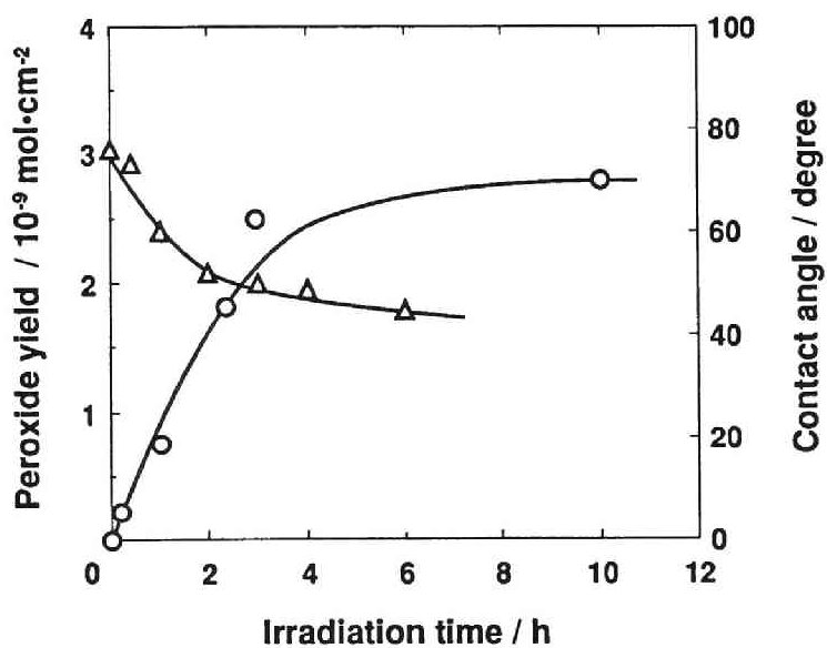
Fig. 2. Various of peroxide yield and contace angle as a function of UV irradiation time: (○) peroxide yield, (Δ) contact angle.
