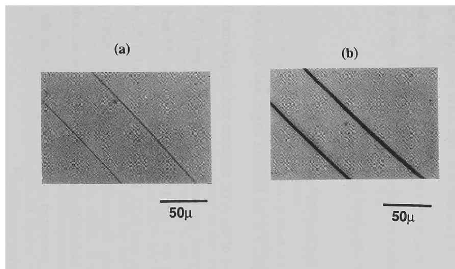
Fig. 8. Optical photographs of the cross-section of PET films stained with Direct Sky Blue 6B. (a) virgin, (b) grafted with PEM-4 to 20 μg·cm -2
