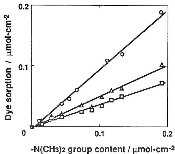
Fig. 8. Effect of the -N(CH 3 ) 2 group content of a DMAEMA-grafted PET film on the sorption of different anions at 30°C and pH 3 for 1 h: (○) mono-SO 3 , (Δ) di-SO 3 , (□) tri-SO 3 .
