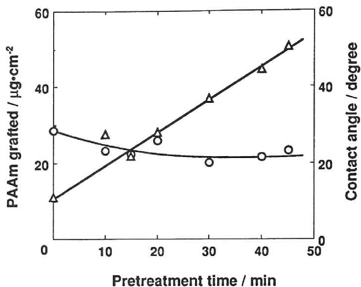
Fig. 4. Effect of pretreatment of PET films with benzyl alcohol on grafting (135 °C, 3 atm): ( \Delta ) graft amount, (O) contact angle.
