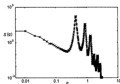
Figure 2: Spatial power spectrum of \partial_r \arg(X_2/X_1) .
