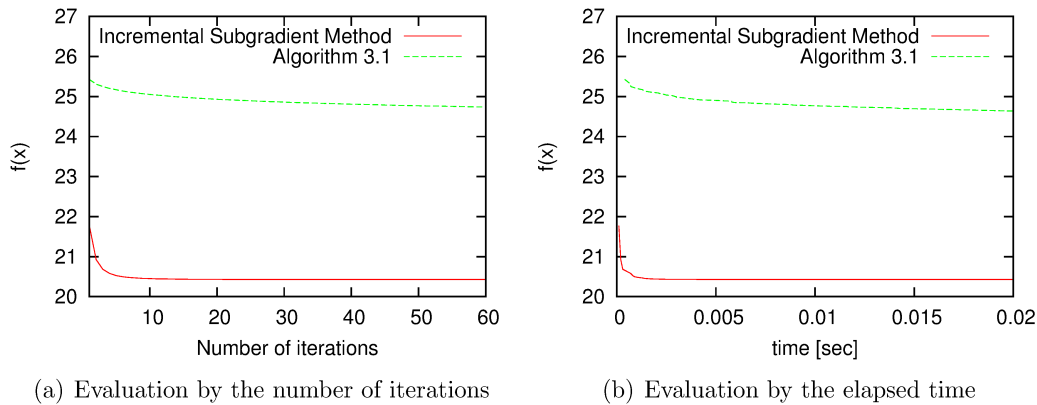
FIGURE 2. Behavior of f(x) with diminishing step size
