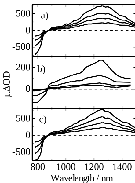
Figure S4. Transient absorption spectra of PCPDTBT/PCBM blend films with different PCBM fractions: a) 5, b) 30, and c) 50 wt% of PCBM. The delay times are 0.5, 1, 2, and 5 \mu\text{s} after the laser excitation at 400 nm with a fluence of 30 \mu\text{J cm}^{-2} .
