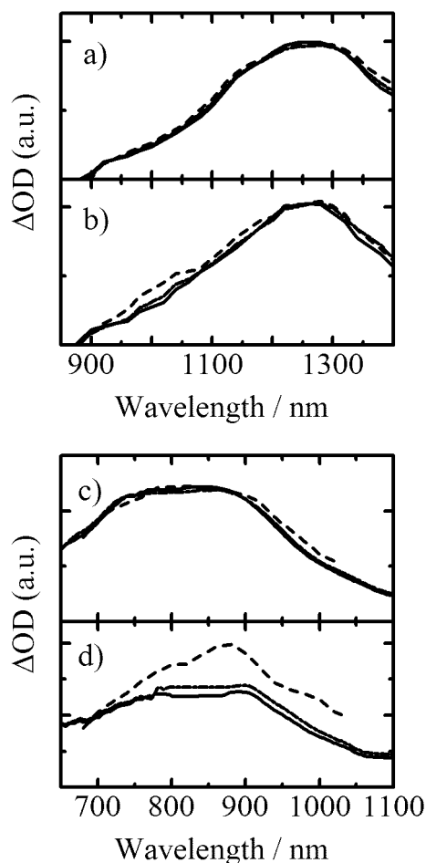
Figure 3. Transient absorption spectra of blend films excited at 400 nm with a fluence of 30 \mu\text{J cm}^{-2} : a) PCPDTBT/PCBM (95 : 5 w/w), b) PCPDTBT/PCBM (50 : 50 w/w), c) N-P7/PCBM (95 : 5 w/w), and d) N-P7/PCBM (50 : 50 w/w). These spectra are normalized at a) and b) 1240 nm and at c) and d) 700 nm. In the panels a) and b), the solid, dashed-dotted, and broken lines show the spectra at 0.5, 2, and 5 \mu\text{s} , respectively. In the panels c) and d), the solid, dashed-dotted, and broken lines show the spectra at 1, 3, and 500 ns, respectively.
