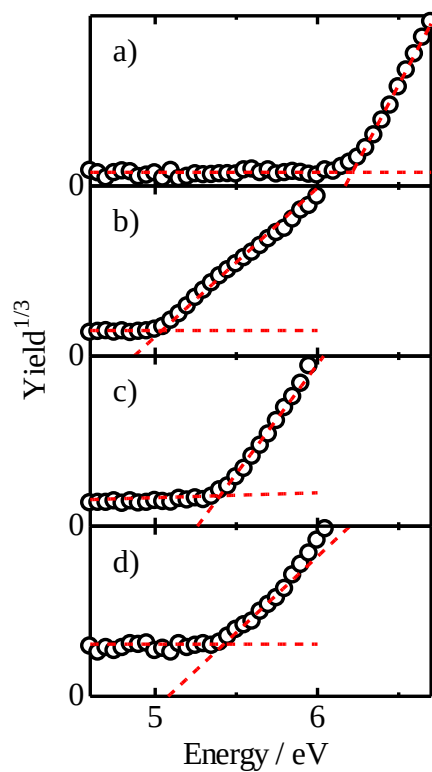
Figure S3. Plots of the cubic root of the photoelectron yields of a) PCBM, b) PCPDTBT, c) N-P7, and d) MDMO-PPV.
