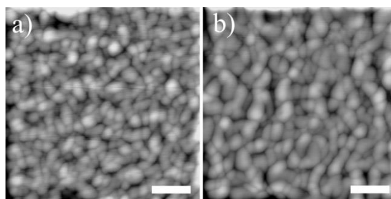
Figure S5. The AFM topographic image of PCPDTBT/PCBM blend films (50 : 50 w/w) measured in the dynamic mode: a) without and b) with 1,8-diiodooctane. These films were washed by 1,8-octanedithiol to remove PCBM. The scale bars correspond to 100 nm in length.
