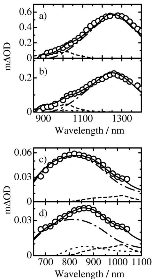
Figure 4. Transient absorption spectra of blend films (open circles) at 1 \mu s after the laser excitation at 400 nm with a fluence of 30 \mu J cm -2 : a) PCPDTBT/PCBM (95 : 5 w/w), b) PCPDTBT/PCBM (50 : 50 w/w), c) N-P7/PCBM (95 : 5 w/w), and d) N-P7/PCBM (50 : 50 w/w). The solid lines represent the absorption spectra simulated by the sum of each absorption spectrum of charge carriers: polymer + (dashed-dotted lines), PCBM - (broken lines), and PCBM + (dotted lines). The mole fraction of each spectrum is as follows: polymer + : PCBM + : PCBM - = a) 50 : 0 : 50, b) 35 : 15 : 50, c) 50 : 0 : 50, and d) 30 : 20 : 50.
