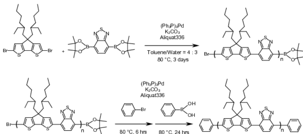
Figure S1. Synthesis scheme of PCPDTBT.
