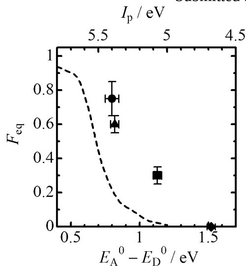
Figure 7. Equilibrium fraction of of PCBM radical cation F_{eq} obtained from the transient study plotted against E_A^0 - E_D^0 (lower axis) and I_p of conjugated polymers (upper axis): MDMO-PPV/PCBM (circle), N-P7/PCBM (triangle), PCPDTBT/PCBM (square), and P3HT/PCBM (diamond) blends. The broken line indicates the calculated F_{eq} with \Delta = 0 shown in Figure 6 for the polymer/fullerene blend with a high fullerene fraction.
