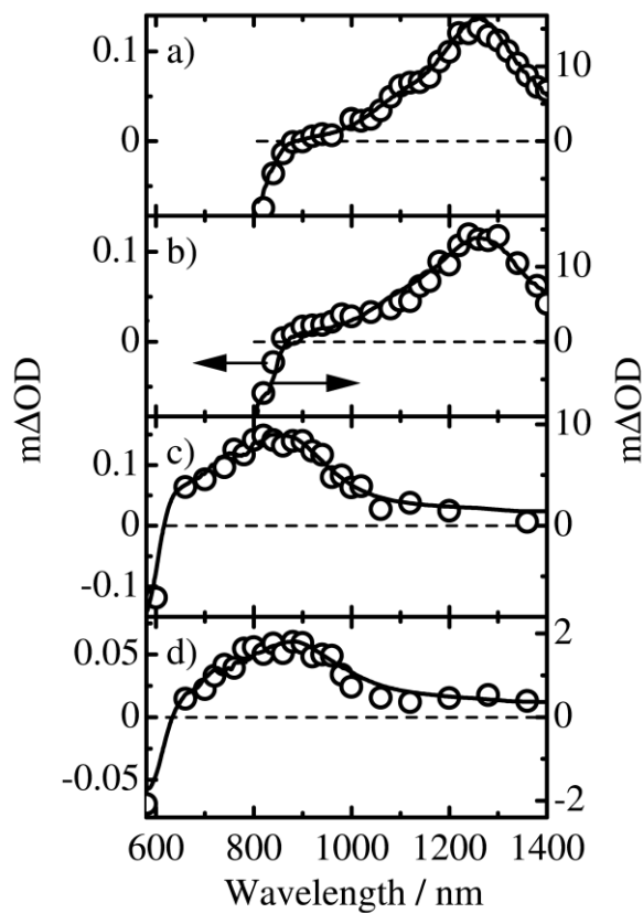
Figure 2. Transient absorption spectra of blend films: a) PCPDTBT/TCNB (95 : 5 w/w), b) PCPDTBT/TCNB (70 : 30 w/w), c) N-P7/TCNB (95 : 5 w/w), and d) N-P7/TCNB (70 : 30 w/w). The solid lines and open circles show the spectra measured at 3 ns and 0.5 \mu s after the laser excitation, respectively. The broken lines represent the baseline.
