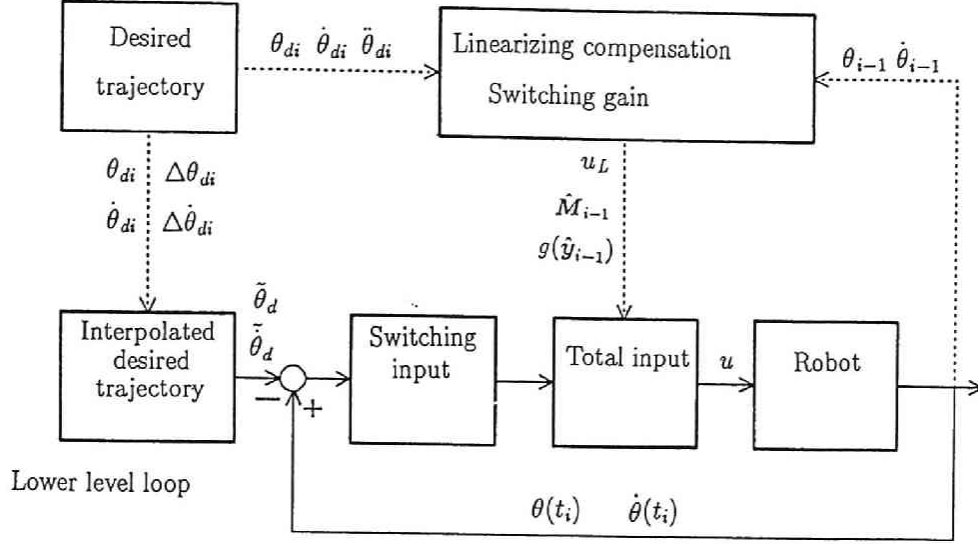
Figure 6.1: Hierarchical robust control system
