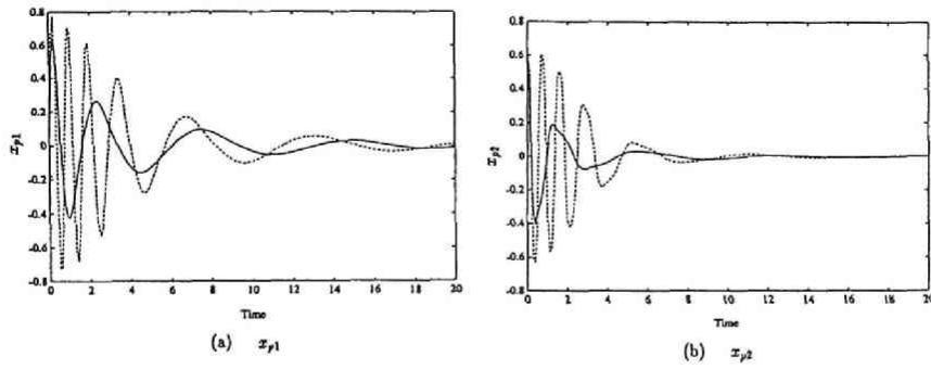
Figure 8.3: Initial state response: (a) x_{p1} , (b) x_{p2} , Solid lines express the nonlinear case, while dashed lines express the linear case
