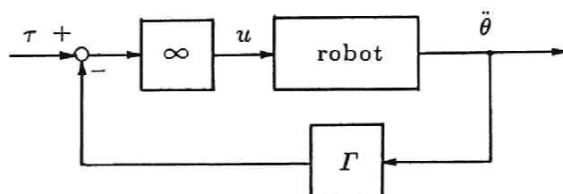
Figure 3.2: Equivalent control system
