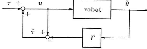
Figure 3.1: Conventional control system
