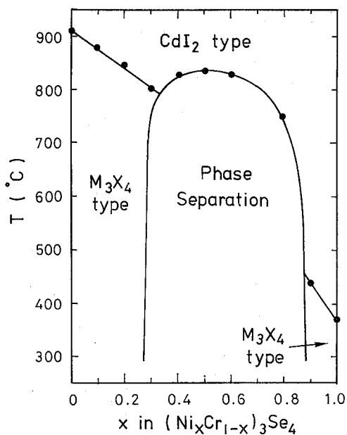
Fig. 15. Phase diagram of the (\text{Ni}_x\text{Cr}_{1-x})_3\text{Se}_4 system
