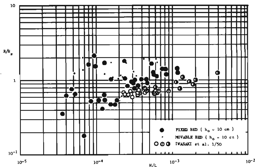
Fig. 6. Run-up referred to H_s as a function of wave steepness ( H/L ).
