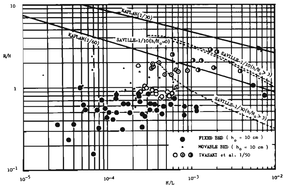
Fig. 5. Run-up ( R/H ) as a function of wave steepness ( H/L ).
