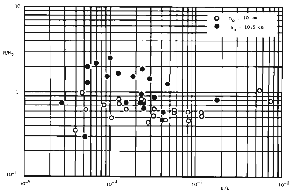
Fig. 8. Effect of water depth in the relation between (R/H_2) and (H/L) .
