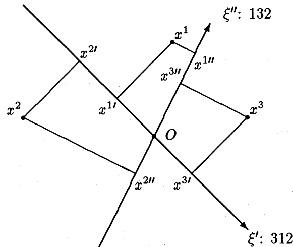
Figure 3: Shapley's construction of orderings
