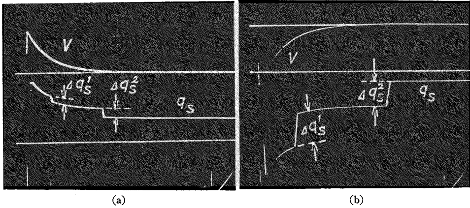
Fig. 14 Probe charge wave form associated with back-discharge. ( \delta=100 mm, 100 \mu\text{s}/\text{div.} )
