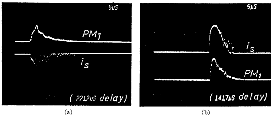
Fig. 13 Current and light pulses associated with back-discharge. ( \delta=100 mm, 5 \mu s/\text{div.} ) (a) By positive impulse. (Applied voltage 150 kV. i_s ; 13.3 mA/div.) (b) By negative impulse. (Applied voltage of -210 kV. i_s ; 13.3 mA/div.)
