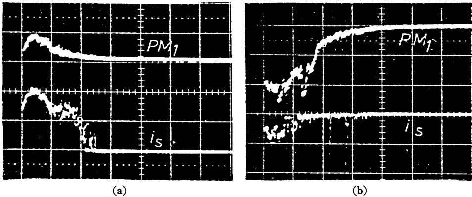
Fig. 11 Current and light pulses associated with A.C. corona. ( \delta=100 mm. Applied voltage 68 kV in R. M. S., i_s ; 6.7 mA/div., 5 \mu\text{s}/\text{div.} )
