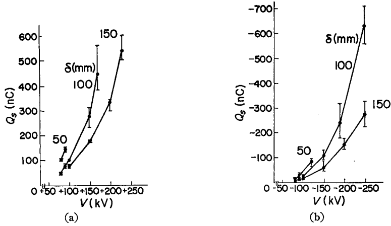
Fig. 6 Relations of corona space charge Q_s vs. impulse voltage V .
