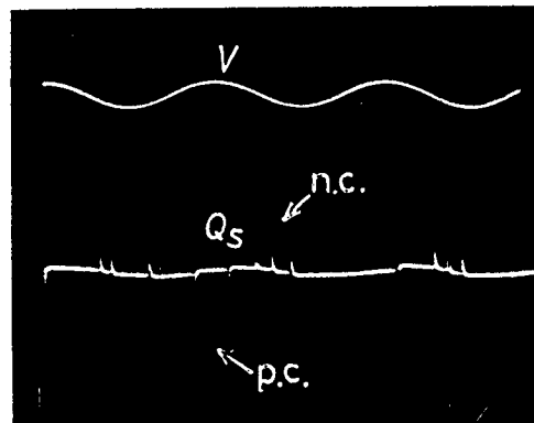
Fig. 8 Wave form of corona space charge for A.C. voltage. ( \delta = 100 mm, Applied voltage 90 kV R.M.S., Q_s ; 133 nC/div., V; 440 kV/div., 5 ms/div.. P.C.; Positive corona, N.C.; negative corona.)
