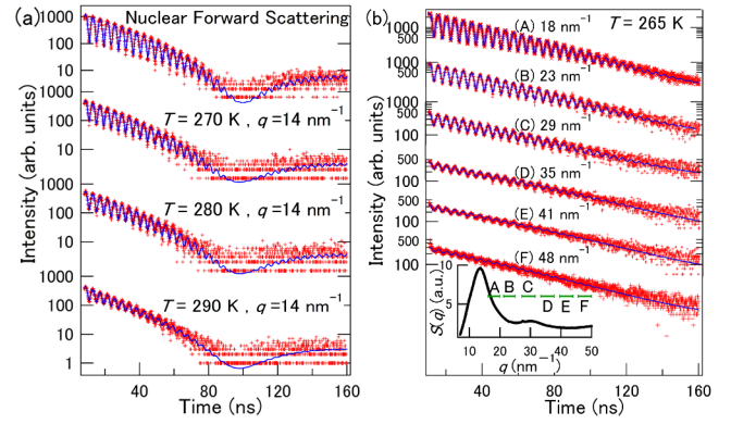
FIG. 1 (color online). Examples of TDI time spectra (+ symbols) and their fitting curves (solid lines) (a) at several T at q = 14 \text{ nm}^{-1} and the nuclear forward scattering spectrum and (b) at several q at 265 K. Inset of (b) shows S(q) (solid line) and the q ranges (bars), which were used for the measurements. The finite size of the q ranges originate from finite solid angles of the detectors. In the measurements, nuclear absorbers of different thicknesses, whose effective thicknesses are about 21 and 10 for the spectra in Figs. 1(a) and 1(b), respectively, were used to optimize the measurement efficiency for the expected relaxation times, and the difference is reflected in the envelope of the time spectra shown in Figs. 1(a) and 1(b).
