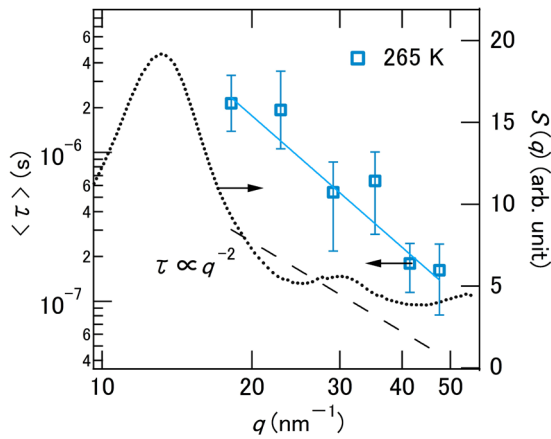
FIG. 3 (color online). q dependence of \langle\tau\rangle at T = 265 K (square symbols) and the static structure factor (dot line). The solid line shows its fitting curve. The dashed line shows the q^{-2} behavior of \langle\tau\rangle .
