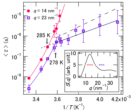
FIG. 2 (color online). T dependence of \langle\tau\rangle at q = 14 and 23 \text{ nm}^{-1} . Solid lines show the fitting curves as discussed in the main text. Short and long dashed lines show the extrapolation of the Arrhenius fitting curve and the dielectric relaxation time of the slow \beta process [22], respectively. The S(q) (solid line) and q regions (bars) used for the measurements are shown in the inset.
