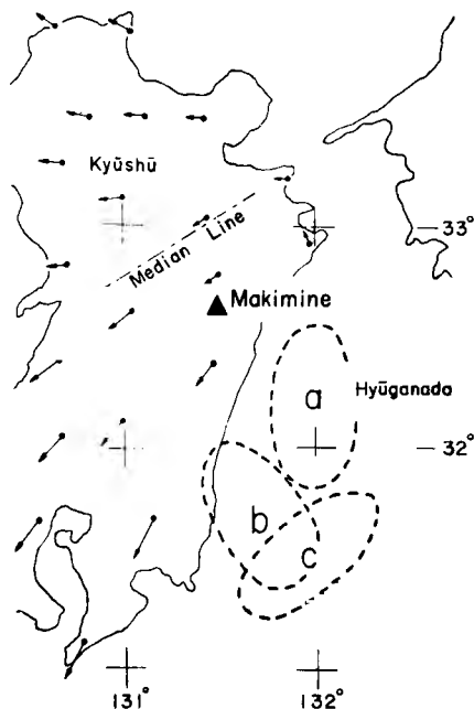
Fig. 3. Originated areas of crustal earthquake sequences ( a , b , c ) and their shifts. Arrows show the directions of horizontal displacements of primary triangulation points.
