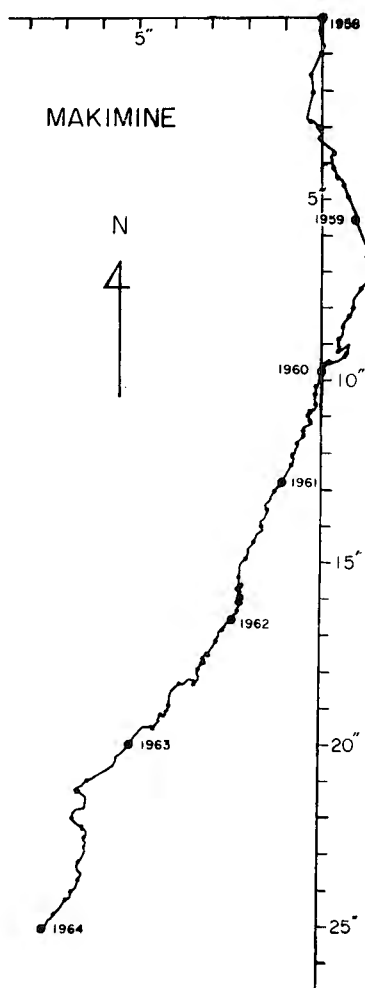
Fig. 1. Vector diagram of ground-tilt observed at Makimine.
