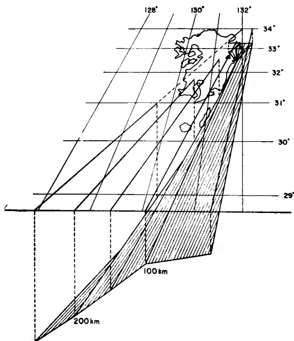
Fig. 6. Supposed surface originating subcrustal earthquake in the northern part of Kyushu-Ryukyû Arc (shown by perspective drawing method).
