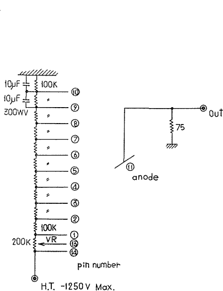
Fig. 8. Divider circuit for a 6655A photomultiplier.
