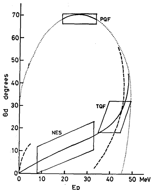
Fig. 2. Proton energies at the cross section maximum as a function of deuteron angle for the ^2\text{H}(d, pd)n reaction at 60 MeV. The solid curves show calculated maxima and areas POF, TQF and NES show the regions mainly produced cross sections through the quasi free scattering of the projectile breakup reaction and the target breakup reaction and through the negative energy scattering. The dashed curves show the kinematical points corresponding to the minimum energies of the spectator neutrons.
