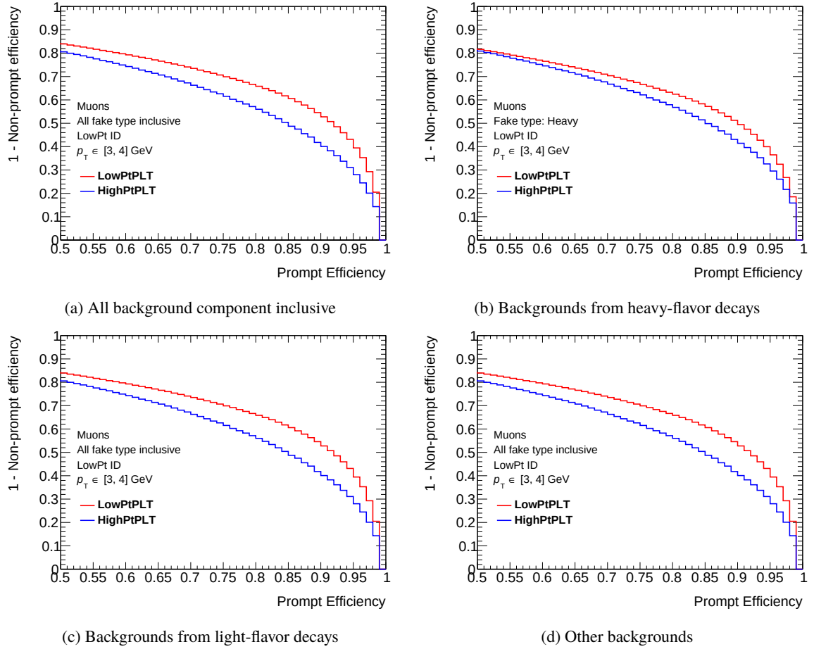
Figure 5.15: ROC curves for LowPtPLT (red lines) and HighPtPLT (blue lines) for muons in p_T \in [3, 4] GeV. The horizontal axis indicate the prompt lepton efficiency, and the vertical axis indicate the rejection of the background leptons, defined by “1 – (background efficiency)”. Different source of the background leptons is considered in each plot; all background source inclusive (top left), heavy-flavor decays (top right), light-flavor decays (bottom left), and other background sources (bottom right). The efficiencies are evaluated using the t\bar{t} MC.
