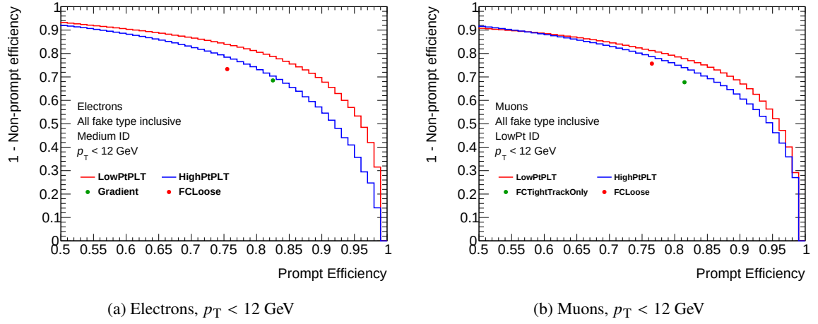
Figure 5.13: ROC curves of the LowPtPLT and HighPtPLT for electrons (left) and muons (right) in the p_T < 12 GeV region. The horizontal axis indicate the prompt lepton efficiency, and the vertical axis indicate the rejection of the non-prompt leptons, defined by “1 – (non-prompt efficiency)”. The red (blue) lines show the ROC curves for LowPtPLT (HighPtPLT). The points indicate the efficiency and the rejection for some of the conventional isolation working points. All the efficiencies are evaluated using the t\bar{t} MC.
