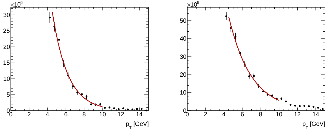
Figure 7.11: The p_T distributions of the muons that pass (left) ID criteria and (right) anti-ID criteria, in fake-factor measurement region with no b -tagged jets. The red line indicates the results of fitting with an exponential function in p_T \in [4.5, 10] GeV. The fitted exponential functions are extrapolated down to 3 GeV to calculate the fake factors in whole p_T range.
